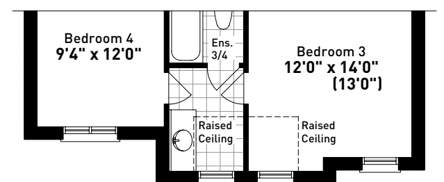
PARTIAL SECOND FLOOR PLAN ELEVATION C
