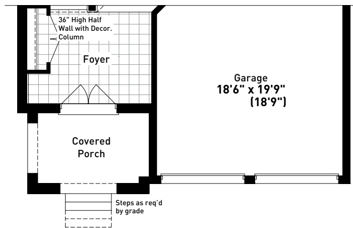
PARTIAL GROUND FLOOR PLAN ELEVATION B
