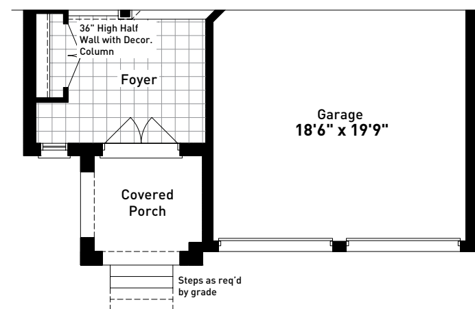
PARTIAL GROUND FLOOR PLAN ELEVATION C
