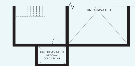
PARTIAL BASEMENT PLAN ELEVATION B
