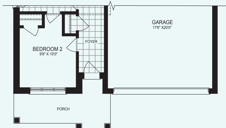
PARTIAL GROUND FLOOR PLAN LOFT B
