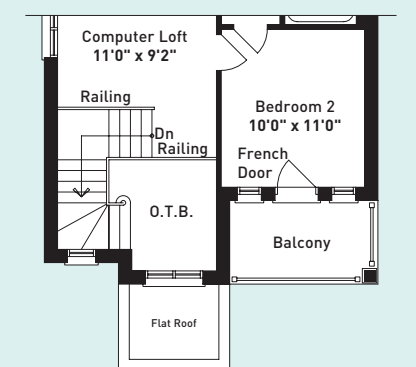
PARTIAL SECOND FLOOR PLAN ELEVATION C
