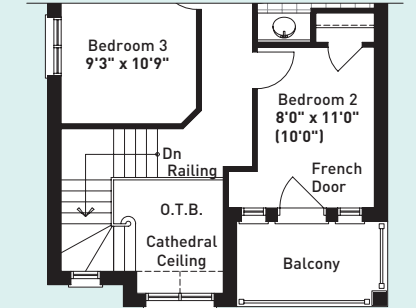
PARTIAL SECOND FLOOR PLAN OPTIONAL 4 BEDROOM ELEVATION B
