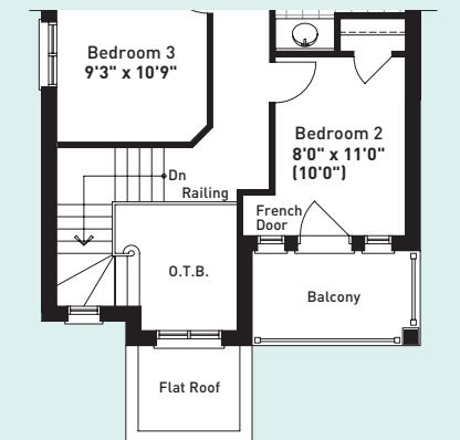
PARTIAL SECOND FLOOR PLAN OPTIONAL 4 BEDROOM ELEVATION C
