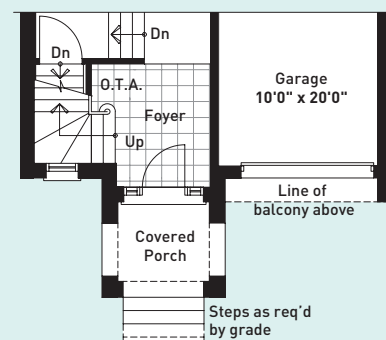
PARTIAL GROUND FLOOR PLAN ELEVATION C
