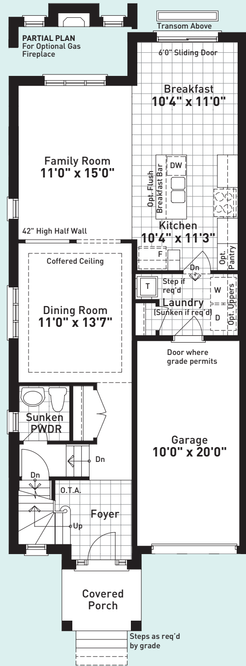
GROUND FLOOR PLAN ELEVATION A
