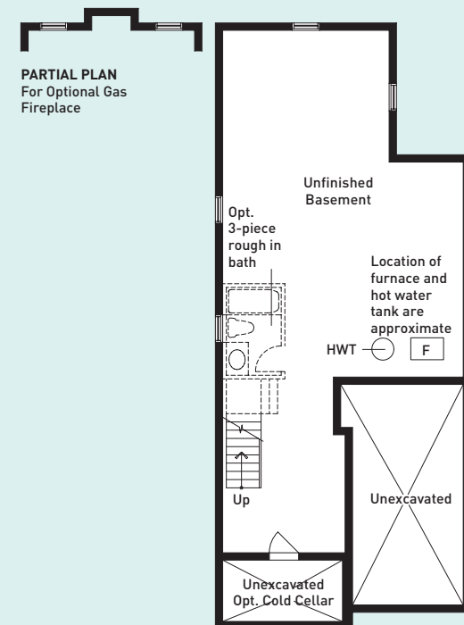
BASEMENT FLOOR PLAN ELEVATION A, B & C
