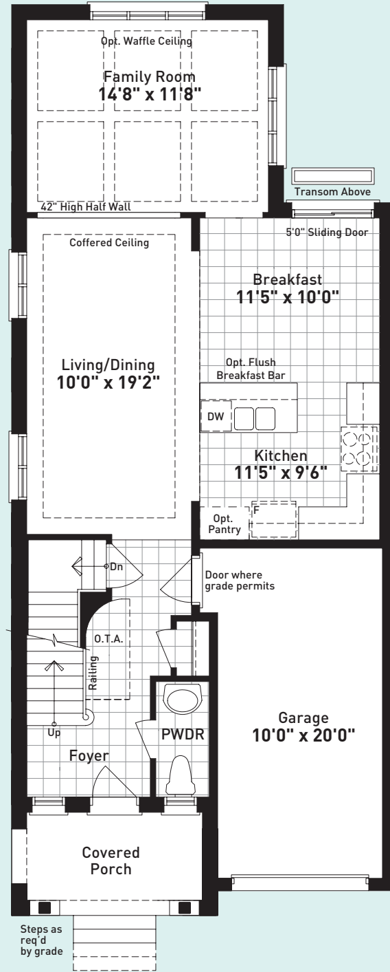
GROUND FLOOR PLAN ELEVATION A
