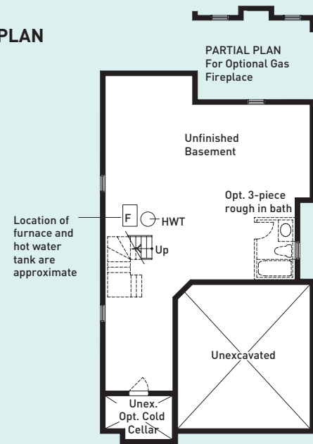
BASEMENT FLOOR PLAN ELEVATION A
