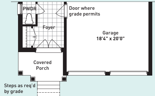
PARTIAL GROUND FLOOR PLAN ELEVATION B
