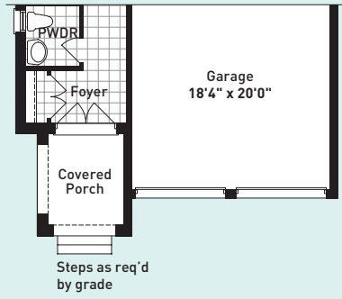
PARTIAL GROUND FLOOR PLAN ELEVATION B
