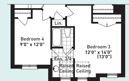
PARTIAL SECOND FLOOR PLAN ELEVATION C
