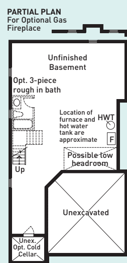
BASEMENT FLOOR PLAN ELEVATION A, B + C
