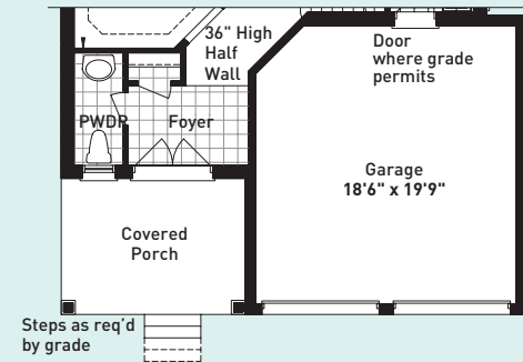
PARTIAL GROUND FLOOR PLAN ELEVATION B
