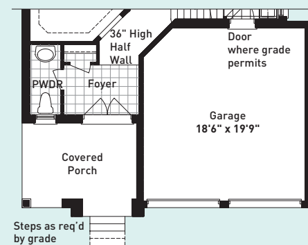
PARTIAL GROUND FLOOR PLAN ELEVATION C
