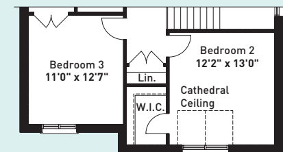
PARTIAL SECOND FLOOR PLAN ELEVATION C
