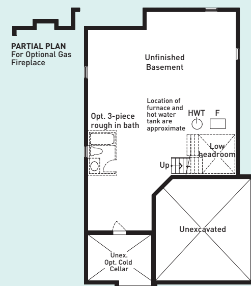
BASEMENT FLOOR PLAN ELEVATION A
