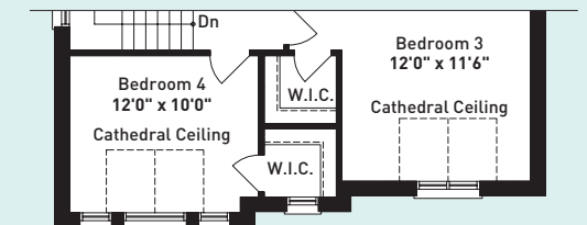
PARTIAL SECOND FLOOR PLAN ELEVATION C
