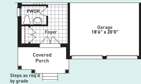
PARTIAL GROUND FLOOR PLAN ELEVATION C
