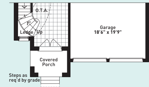
PARTIAL GROUND FLOOR PLAN ELEVATION C
