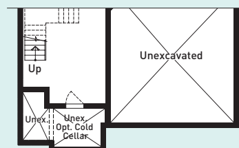
PARTIAL BASEMENT FLOOR PLAN ELEVATION B
