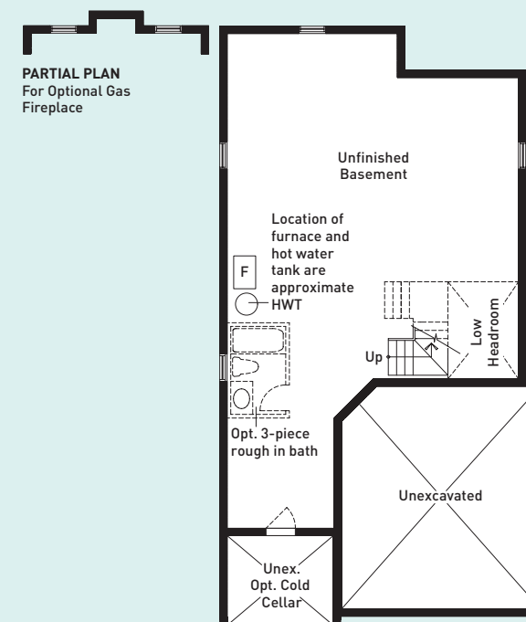
BASEMENT FLOOR PLAN ELEVATION A, B (ELEVATION C SIMILAR)
