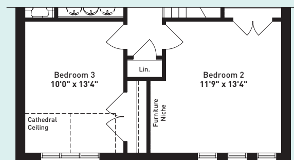
PARTIAL SECOND FLOOR PLAN ELEVATION C
