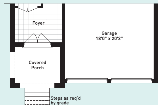
PARTIAL GROUND FLOOR PLAN ELEVATION C
