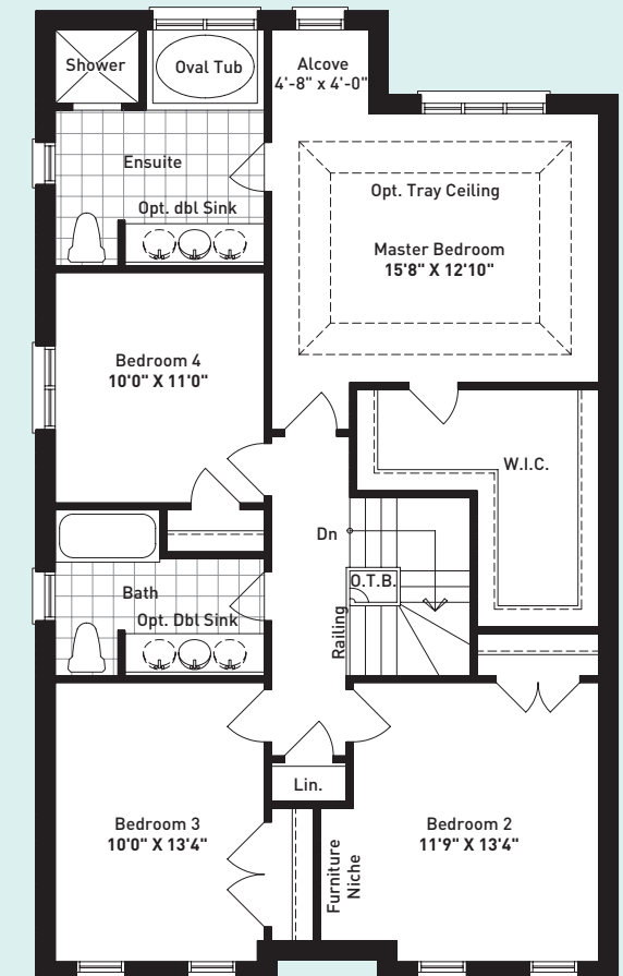
SECOND FLOOR PLAN ELEVATION B
