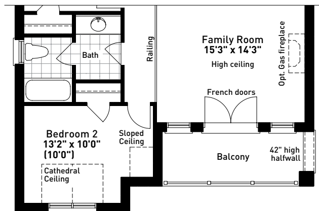
PARTIAL OPT. 4 BEDROOM SECOND FLOOR PLAN ELEVATION C
