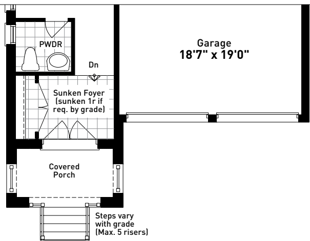
GROUND FLOOR PLAN ELEVATION C
