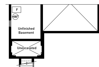
PARTIAL BASEMENT PLAN OPT. / REC. ROOM ELEVATION C
