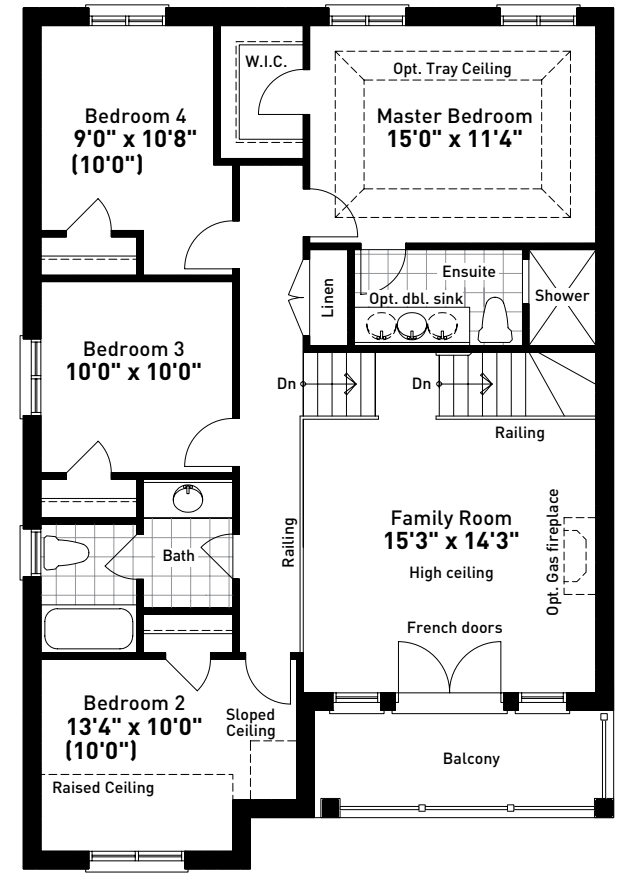
OPT. 4 BEDROOM SECOND FLOOR PLAN ELEVATION B
