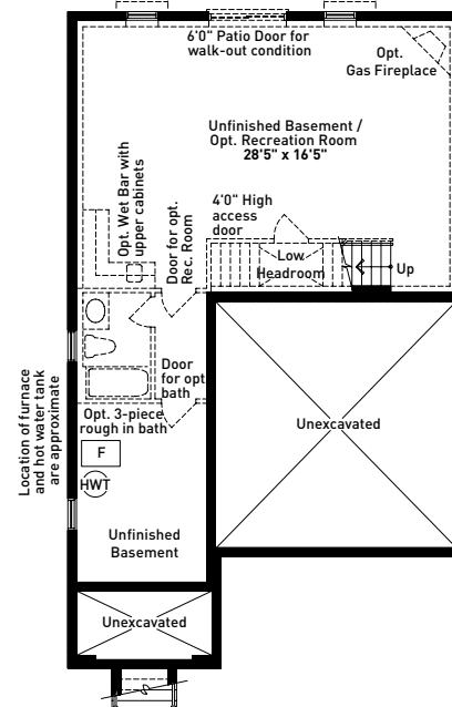
BASEMENT PLAN OPT. / REC. ROOM ELEVATION B
