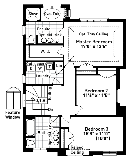
SECOND FLOOR PLAN ELEVATION B
