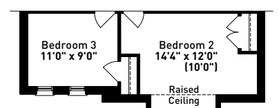
OPT. 4 BEDROOM SECOND FLOOR PLAN ELEVATION C
