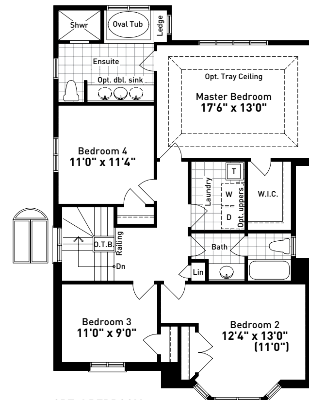
OPT. 4 BEDROOM SECOND FLOOR PLAN ELEVATION A
