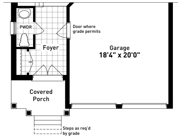
PARTIAL GROUND FLOOR PLAN ELEVATION B
