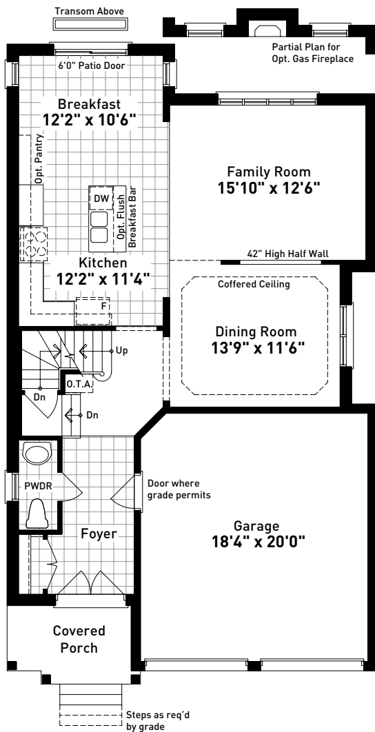
GROUND FLOOR PLAN ELEVATION A
