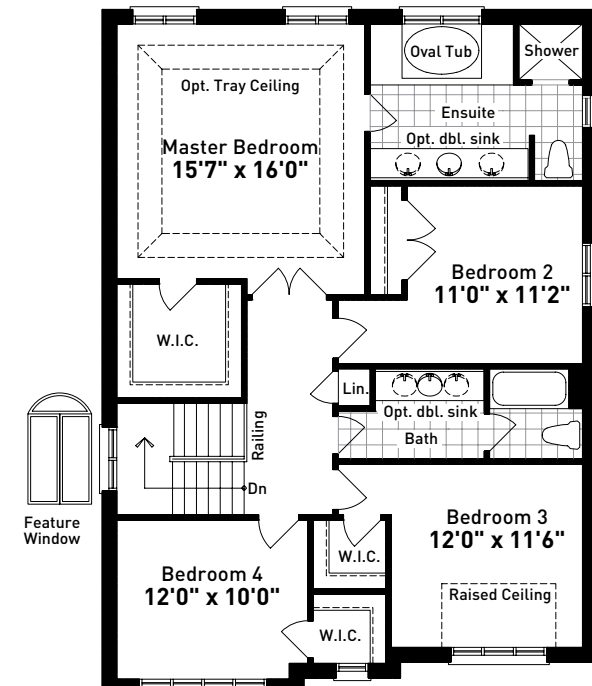
SECOND FLOOR PLAN ELEVATION B
