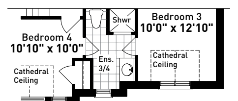
PARTIAL OPTIONAL SECOND FLOOR PLAN ELEVATION C
