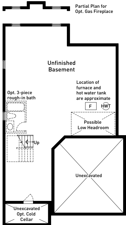
BASEMENT FLOOR PLAN ELEVATION A
