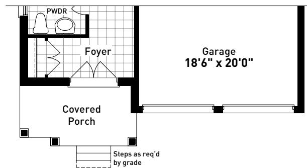
PARTIAL GROUND FLOOR PLAN ELEVATION C
