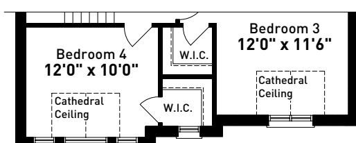
PARTIAL SECOND FLOOR PLAN ELEVATION C
