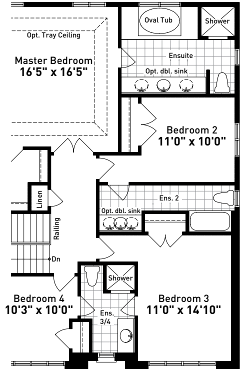
PARTIAL OPTIONAL SECOND FLOOR PLAN ELEVATION A
