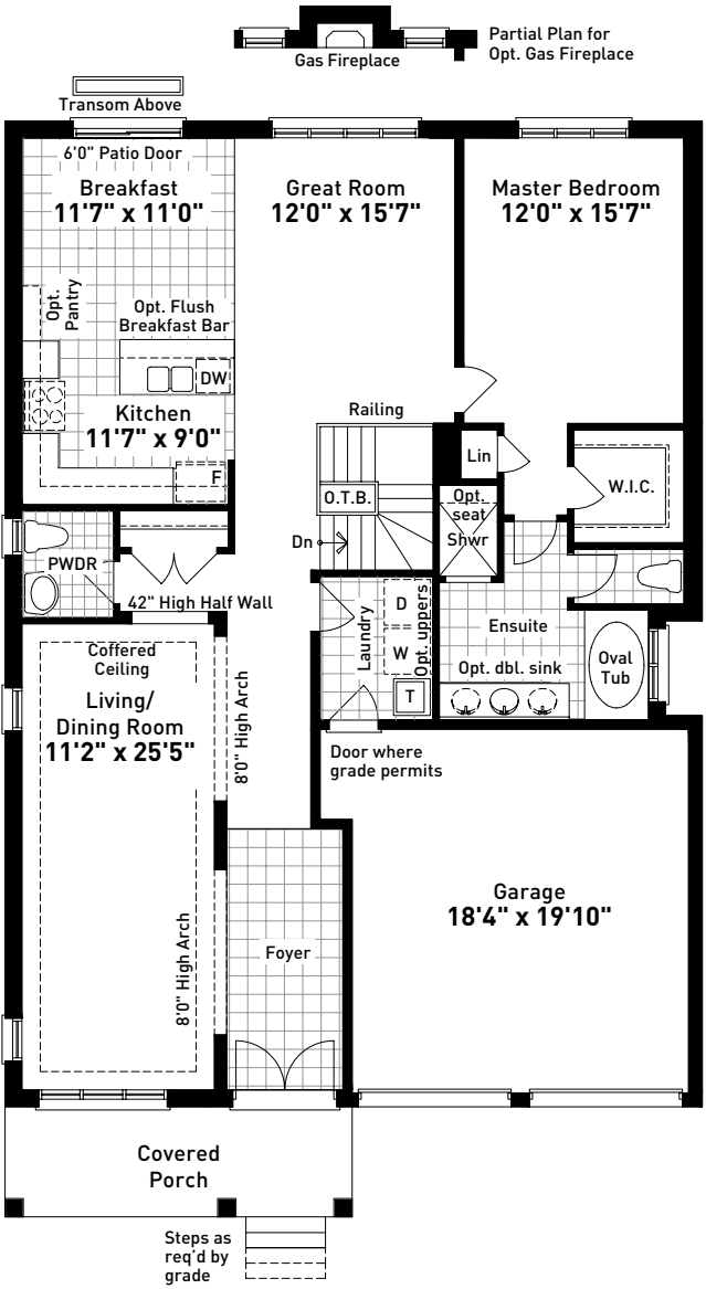
ALTERNATE GROUND FLOOR PLAN BUNGALOW ELEVATION A
