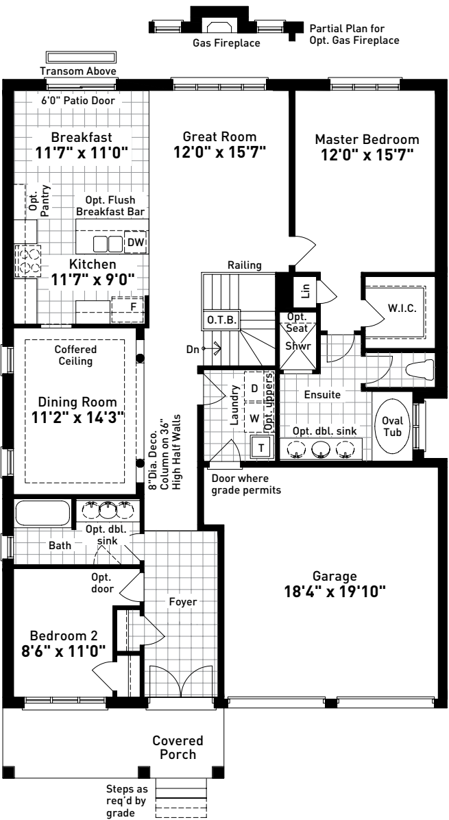
GROUND FLOOR PLAN BUNGALOW ELEVATION A
