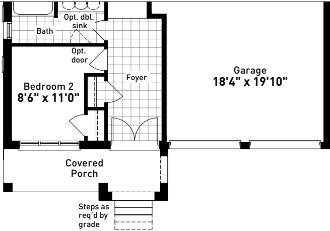
PARTIAL GROUND FLOOR PLAN BUNGALOW ELEVATION B
