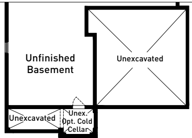
PARTIAL BASEMENT FLOOR PLAN BUNGALOW ELEVATION B
