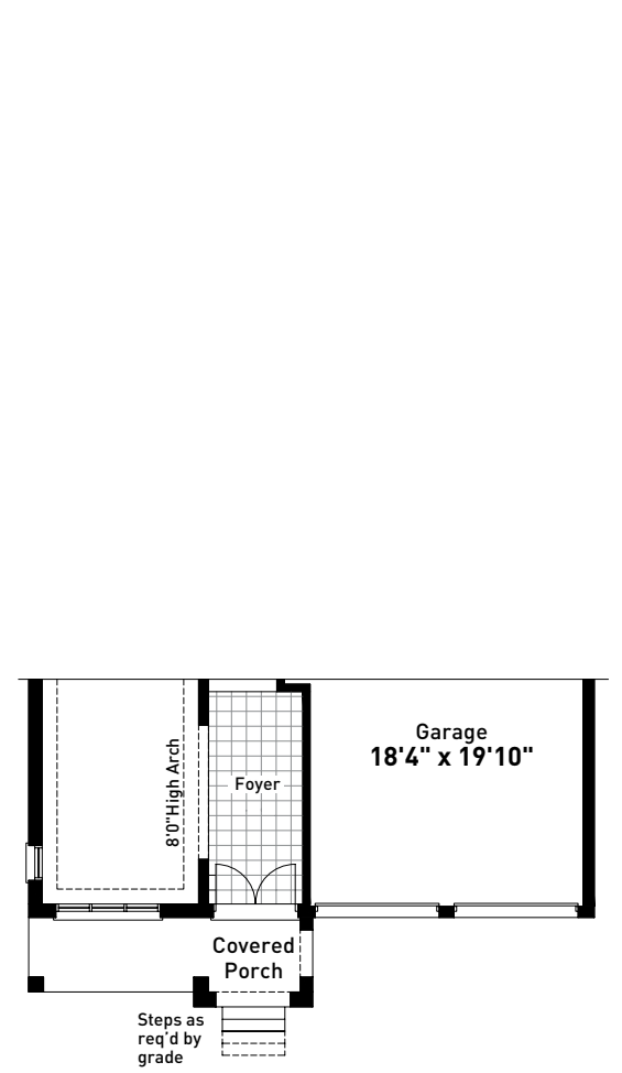
PARTIAL ALTERNATE GROUND FLOOR PLAN LOFT ELEVATION B
