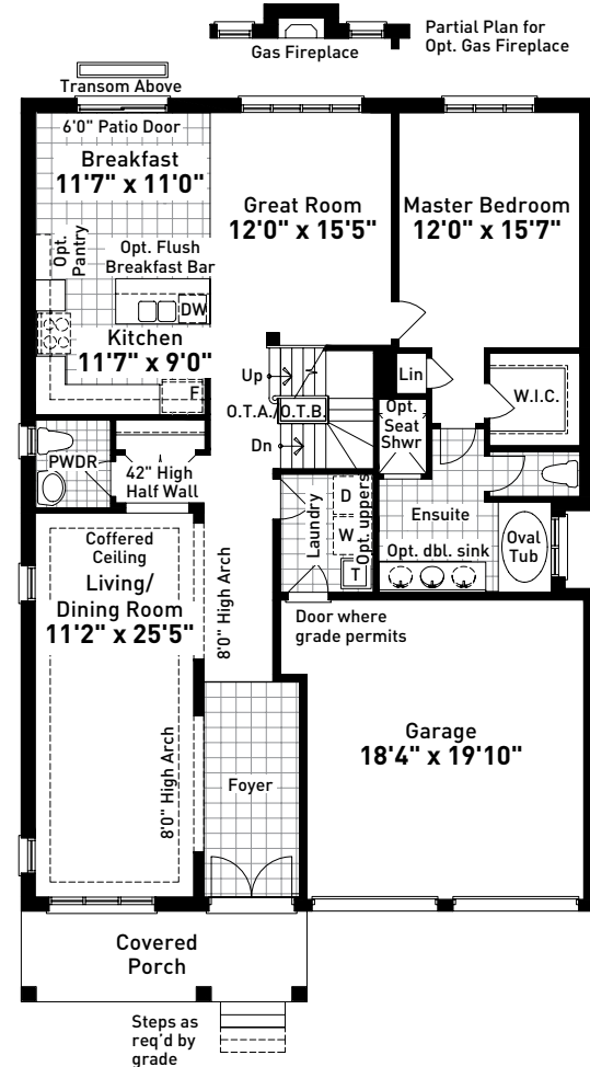
ALTERNATE GROUND FLOOR PLAN LOFT ELEVATION A
