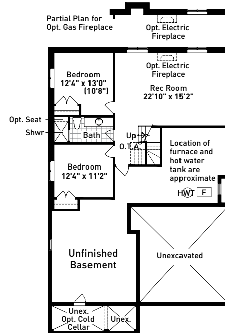
OPT. FINISHED BASEMENT FLOOR PLAN LOFT ELEVATION A
