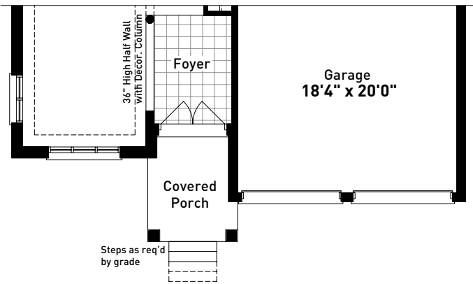
PARTIAL GROUND FLOOR PLAN ELEVATION C
