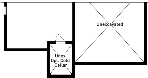
PARTIAL BASEMENT FLOOR PLAN ELEVATION C
