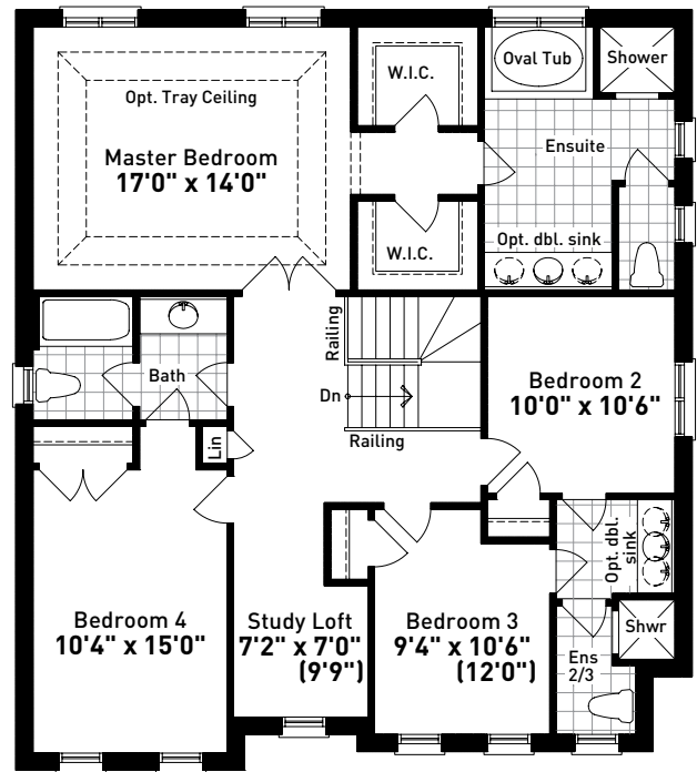
SECOND FLOOR PLAN ELEVATION B
