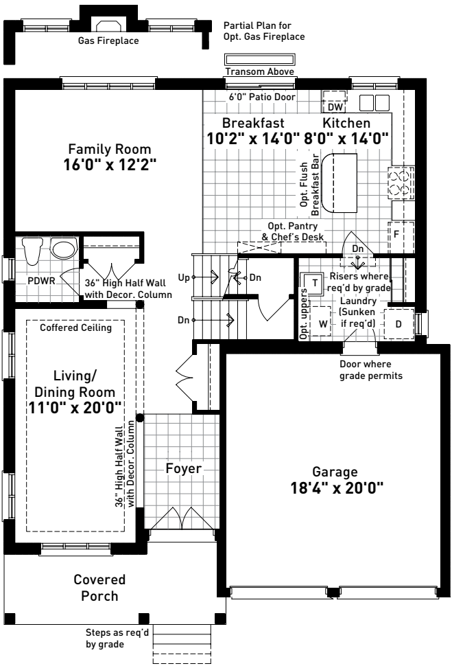
GROUND FLOOR PLAN ELEVATION A
