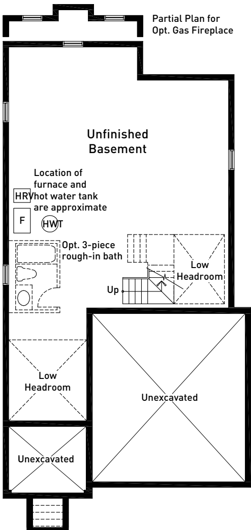
BASEMENT FLOOR PLAN ELEVATION B
