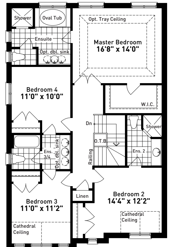
OPT. SECOND FLOOR PLAN WITH BEDROOM 2 ENSUITE ELEVATION C
