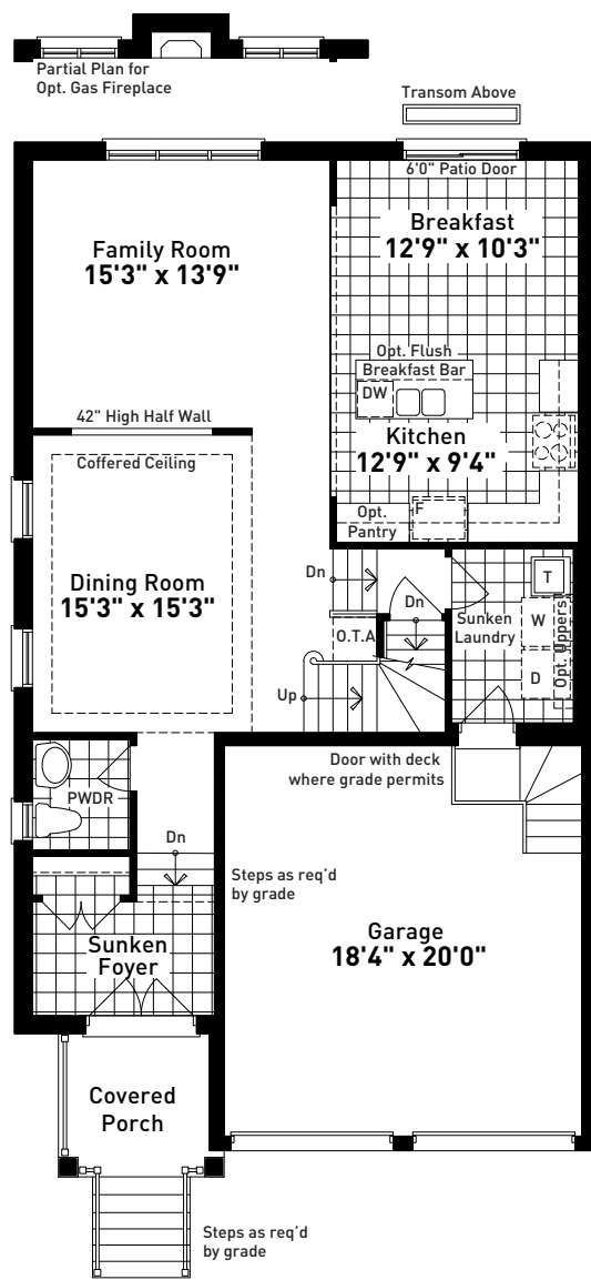
GROUND FLOOR PLAN ELEVATION C
