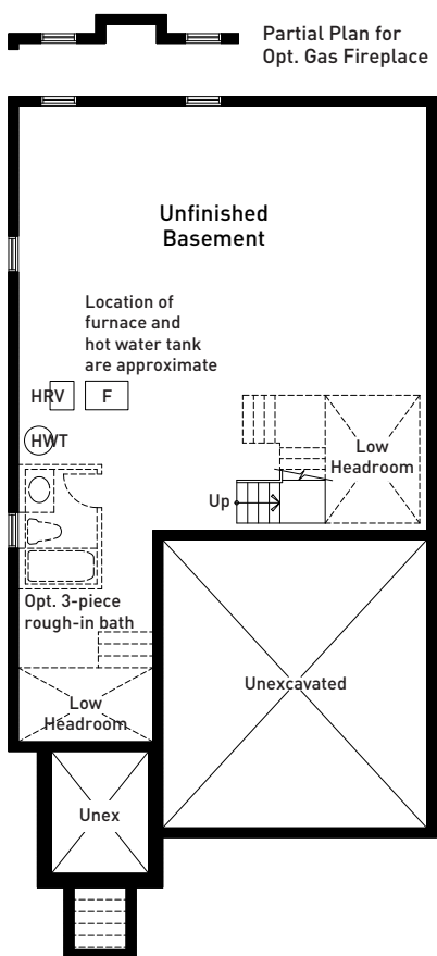
BASEMENT FLOOR PLAN ELEVATION B
