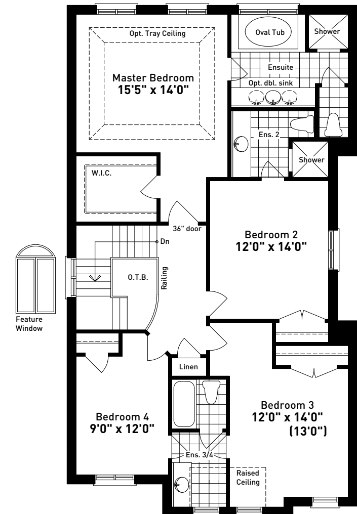
SECOND FLOOR PLAN ELEVATION C
