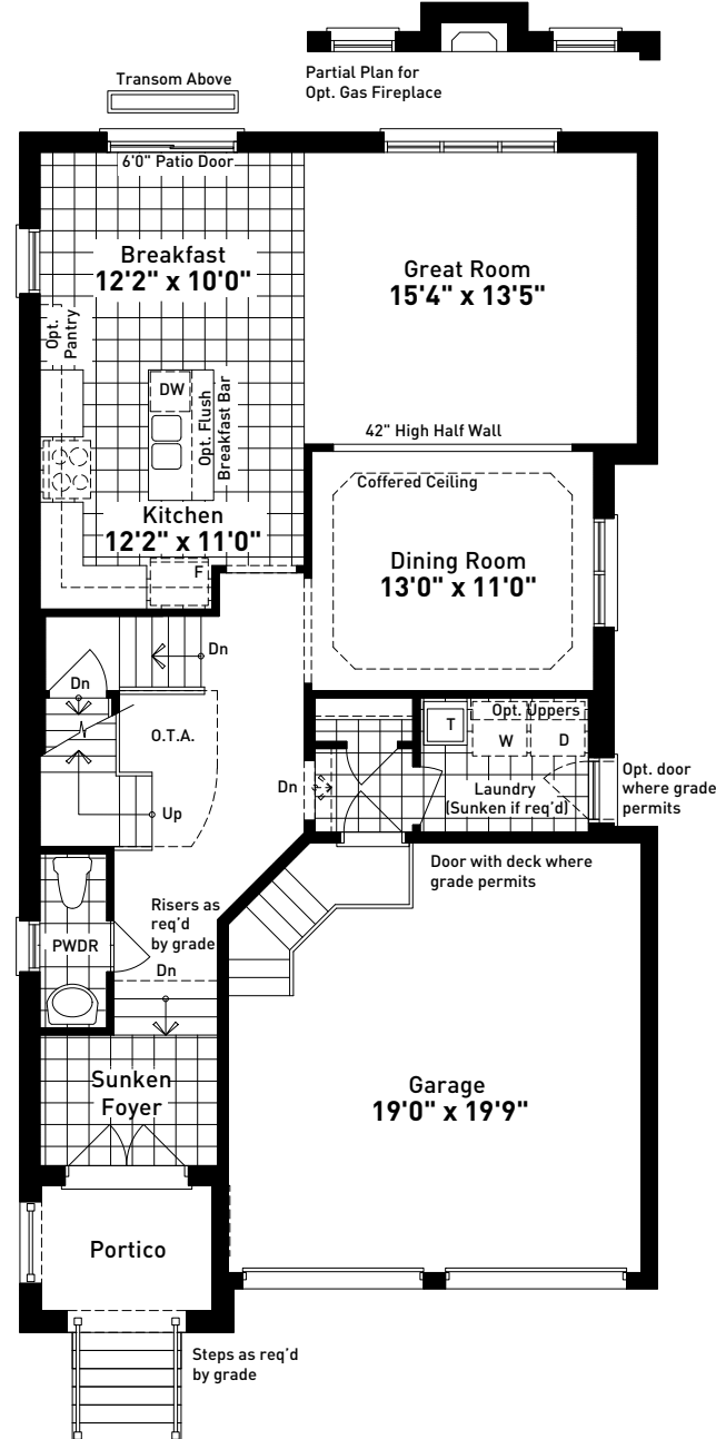
GROUND FLOOR PLAN ELEVATION C
