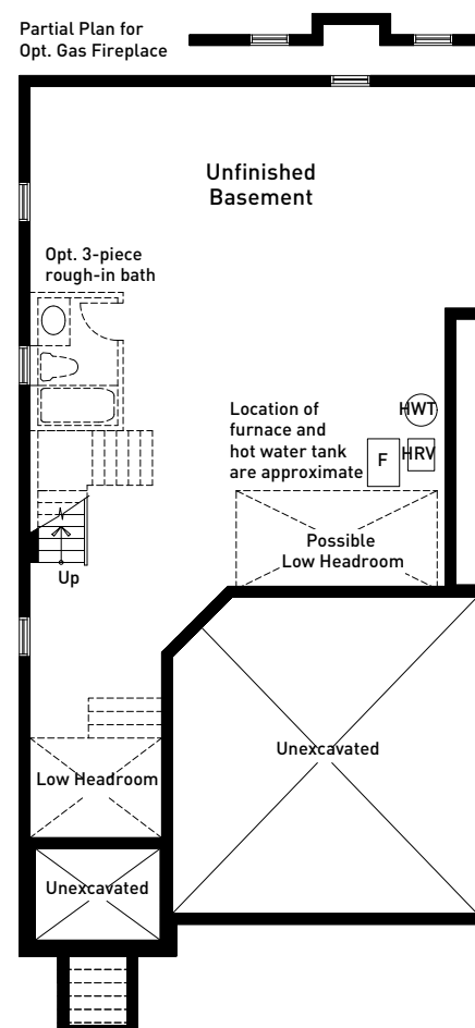
PARTIAL BASEMENT FLOOR PLAN ELEVATION C
