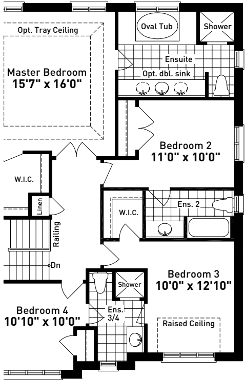
PARTIAL OPTIONAL SECOND FLOOR PLAN ELEVATION B
