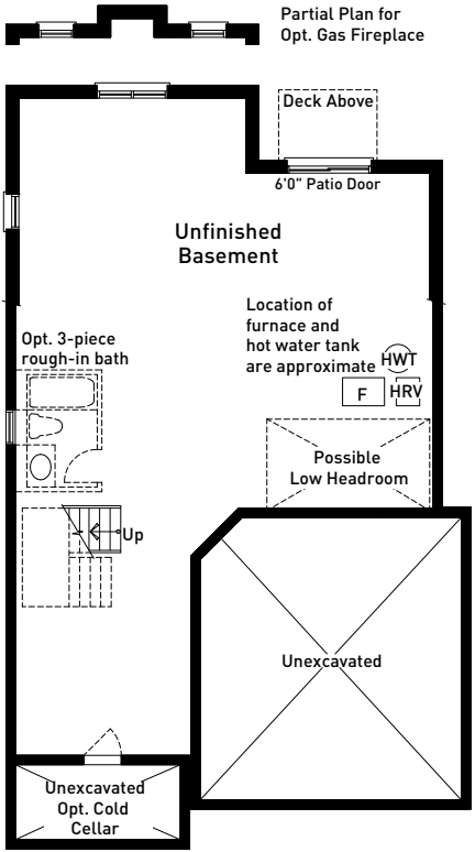
WALKOUT BASEMENT FLOOR PLAN ELEVATION A
