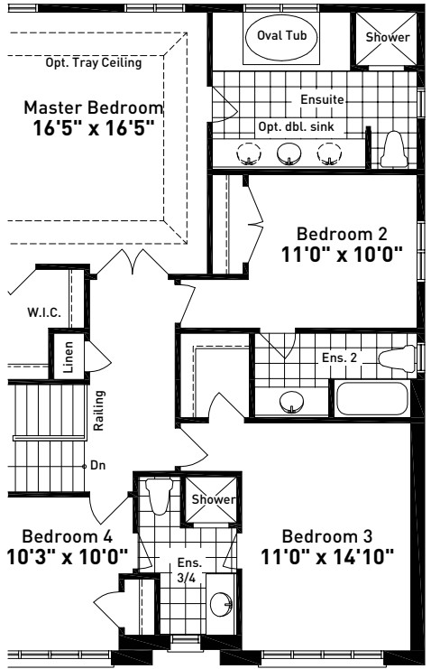
PARTIAL OPTIONAL SECOND FLOOR PLAN ELEVATION A
