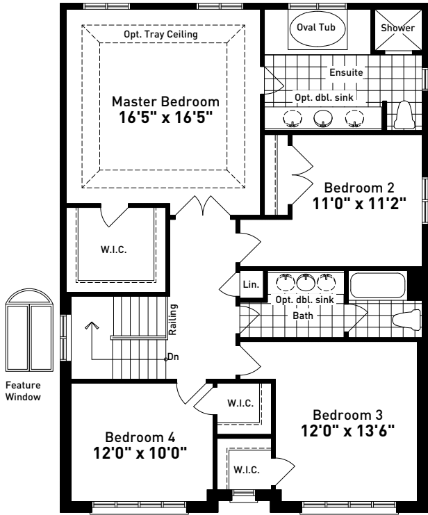
SECOND FLOOR PLAN ELEVATION A
