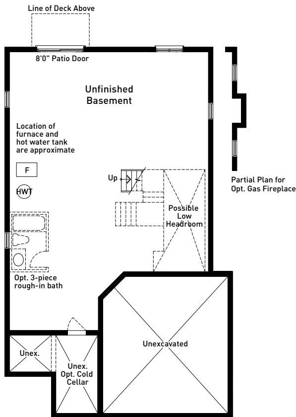
WALKOUT BASEMENT FLOOR PLAN ELEVATION A
