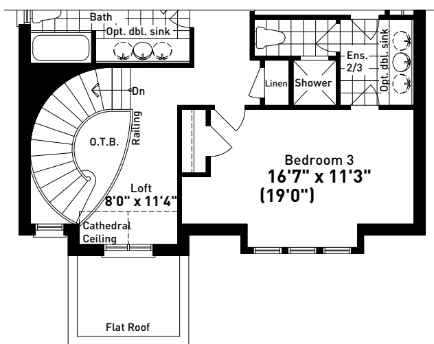
PARTIAL SECOND FLOOR PLAN ELEVATION C
