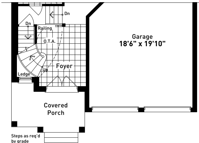
PARTIAL GROUND FLOOR PLAN ELEVATION B
