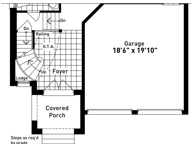
PARTIAL GROUND FLOOR PLAN ELEVATION C
