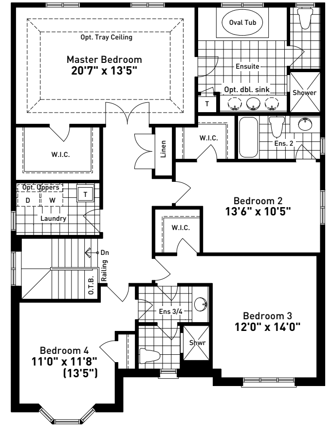
SECOND FLOOR PLAN ELEVATION A
