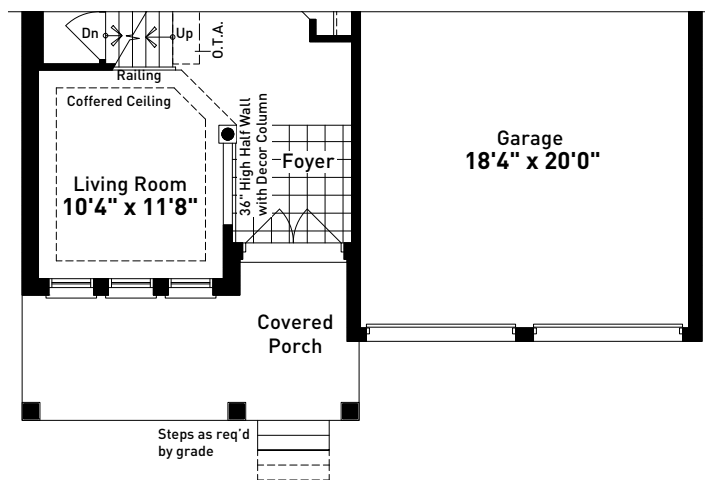
PARTIAL GROUND FLOOR PLAN ELEVATION C
