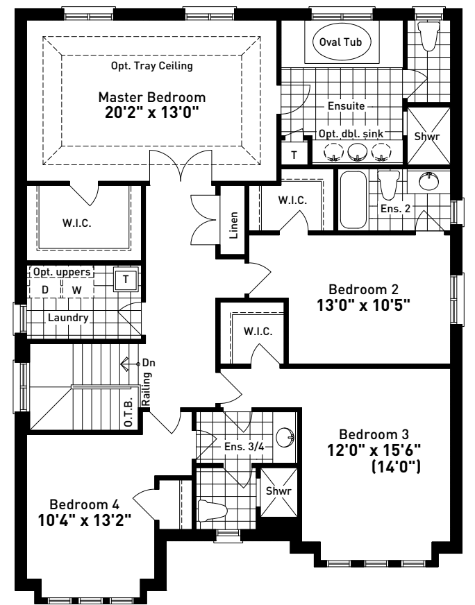
SECOND FLOOR PLAN ELEVATION B
