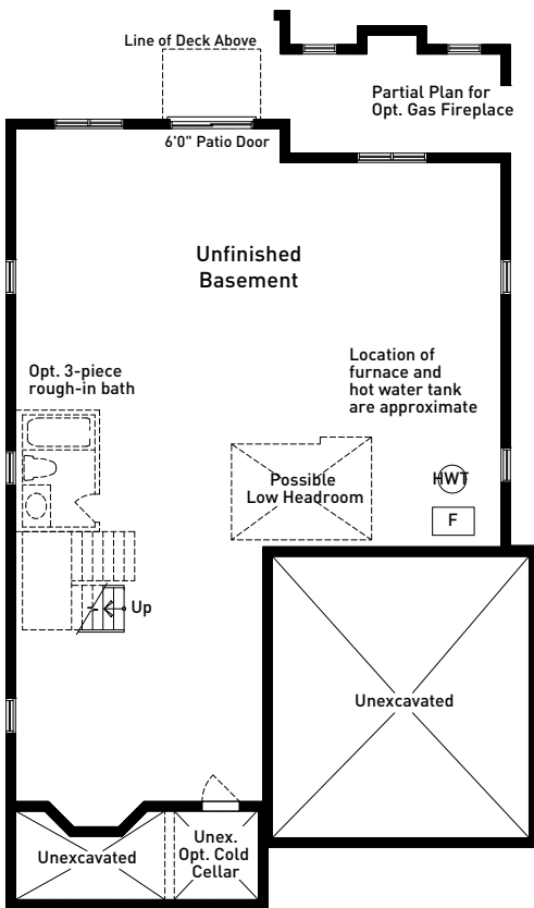
WALKOUT BASEMENT FLOOR PLAN ELEVATION A
