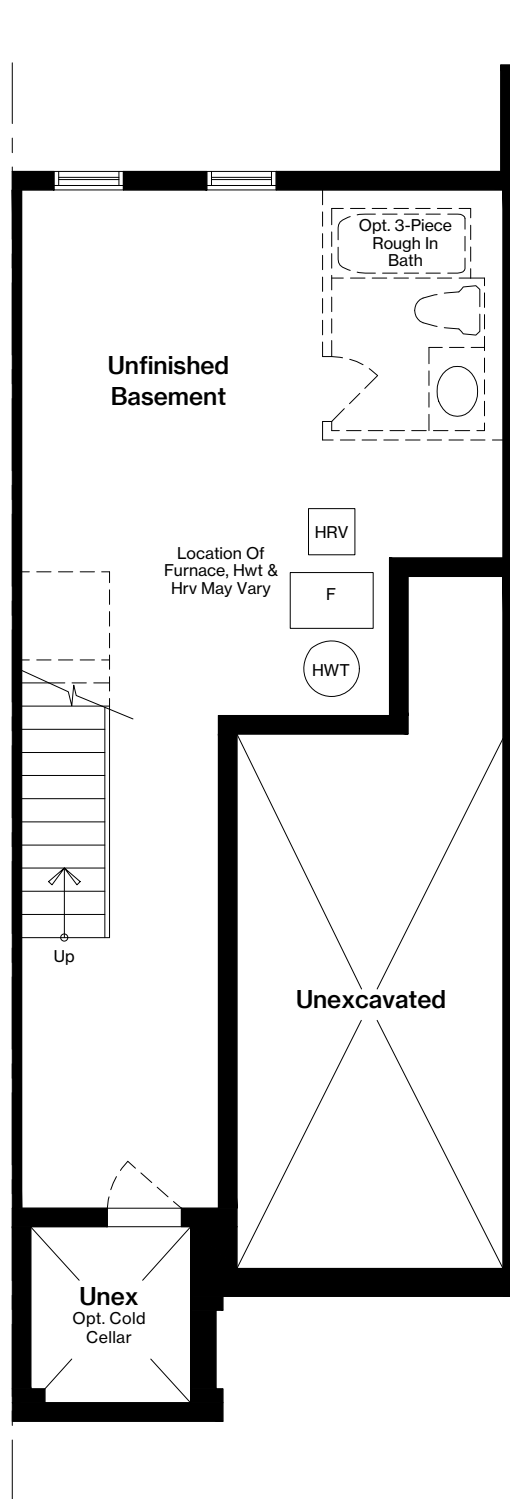
BASEMENT PLAN
