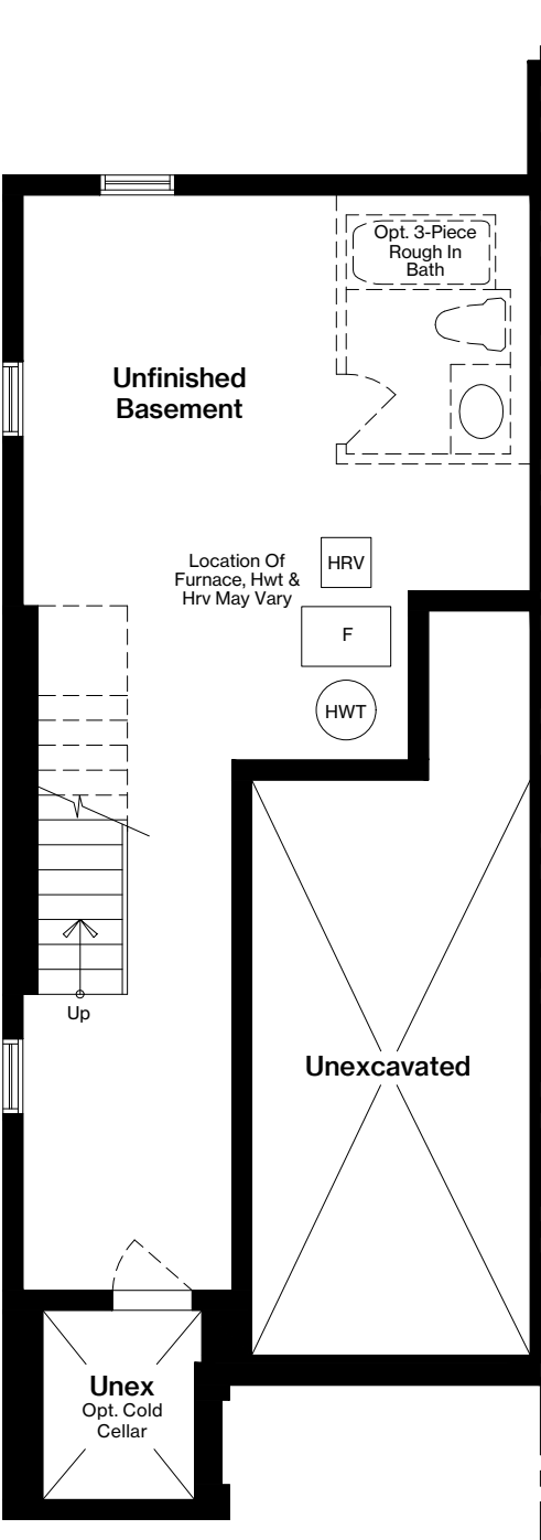
CORNER BASEMENT PLAN
