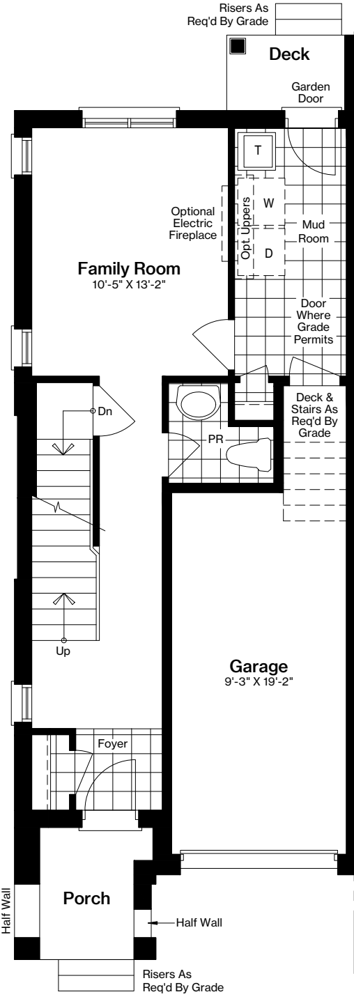
CORNER FIRST FLOOR PLAN
