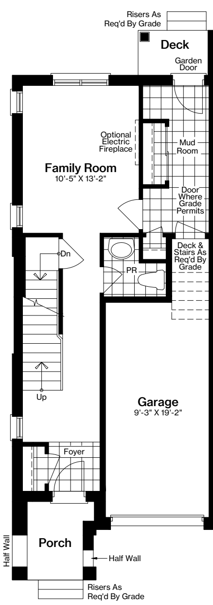
OPTION 4: OPTIONAL SECOND FLOOR LAUNDRY LAYOUT WITH SECOND FLOOR LAUNDRY
