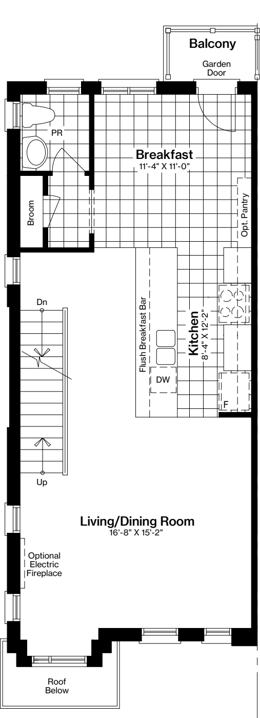
CORNER SECOND FLOOR PLAN
