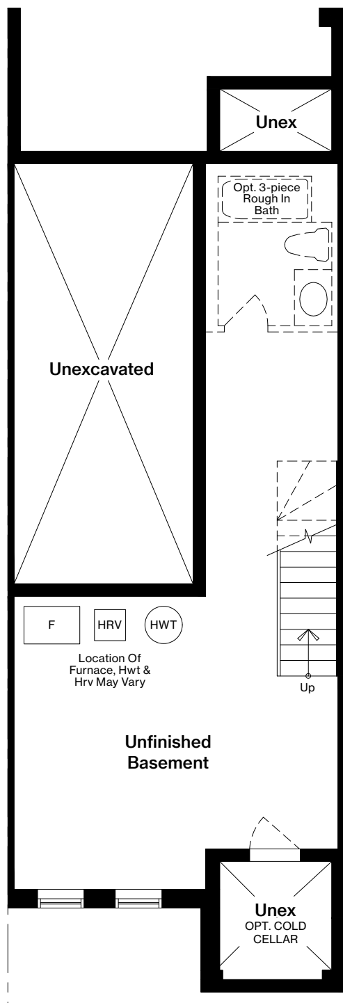
BASEMENT PLAN
