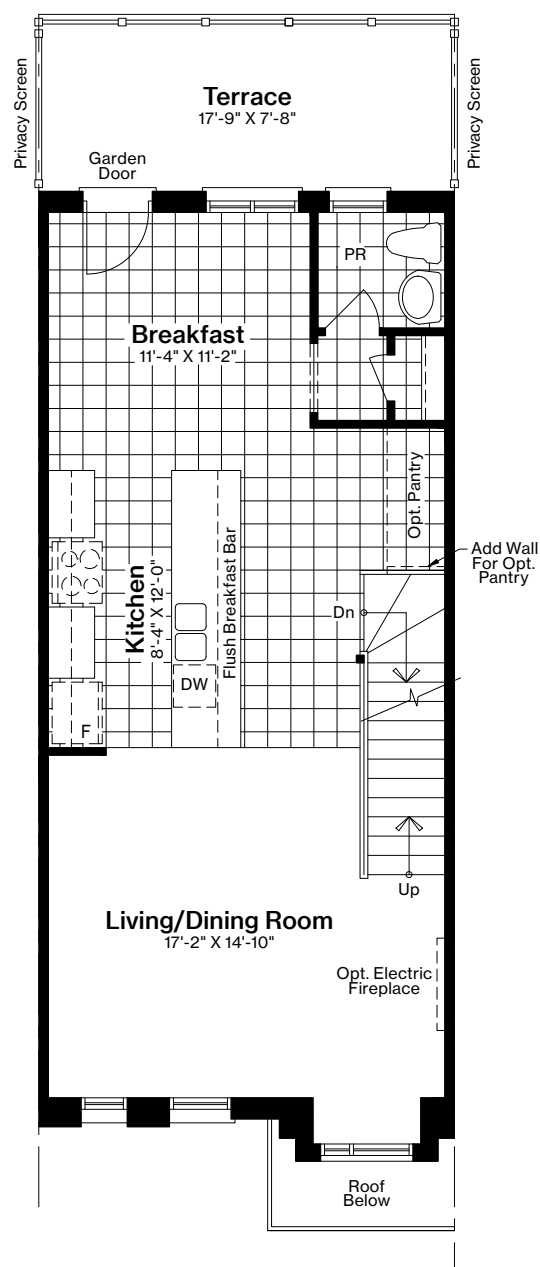
OPTION 2 & 5: ALTERNATE KITCHEN LAYOUT SECOND FLOOR PLAN
