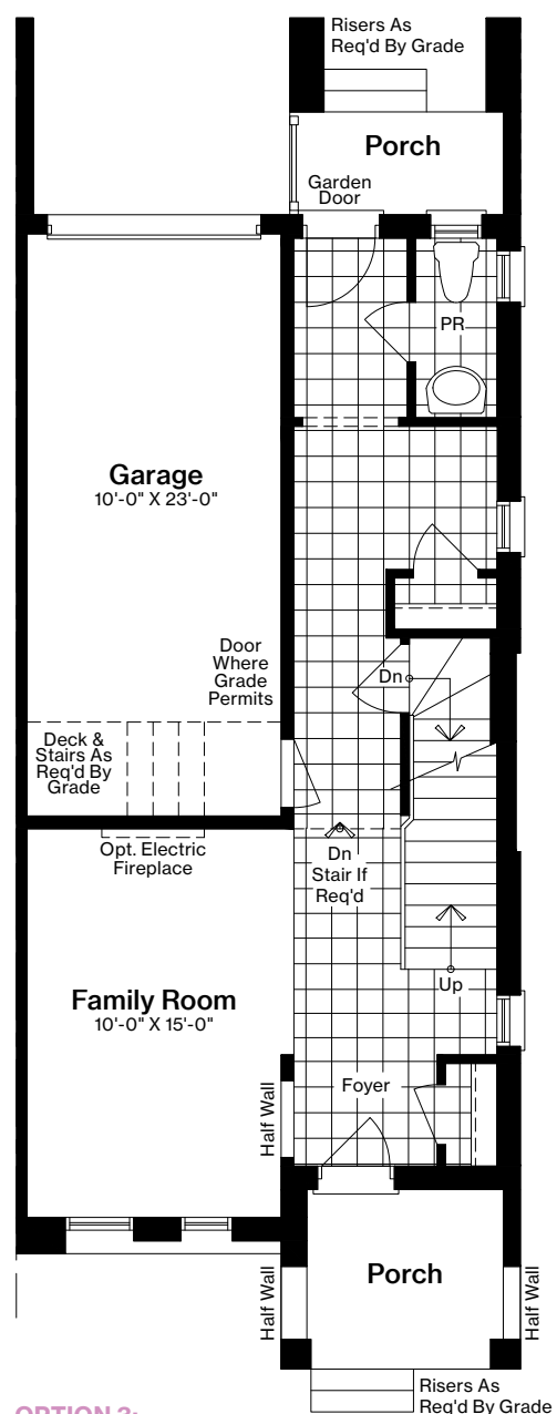
OPTION 3: OPTIONAL SECOND FLOOR LAUNDRY LAYOUT CORNER FIRST FLOOR PLAN
