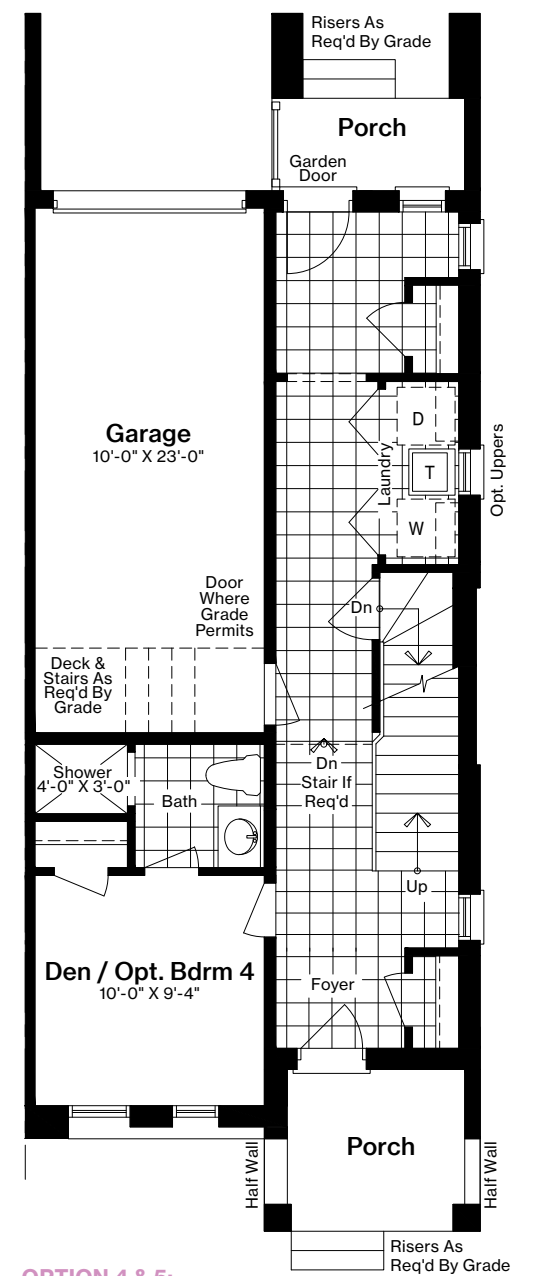
OPTION 4 & 5: OPTIONAL DEN / 4 BEDROOM LAYOUT CORNER FIRST FLOOR PLAN
