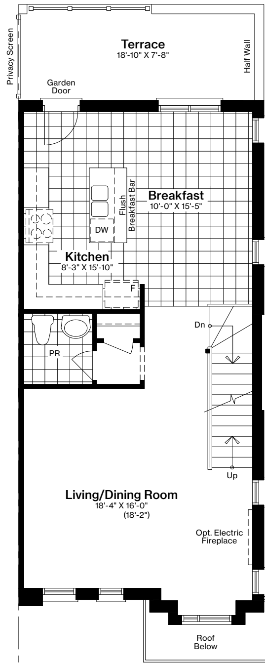
CORNER SECOND FLOOR PLAN
