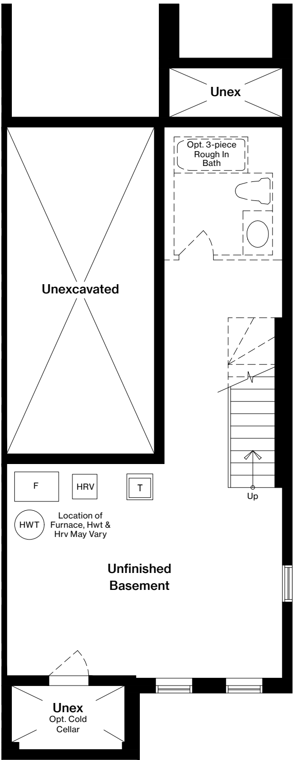
CORNER BASEMENT PLAN
