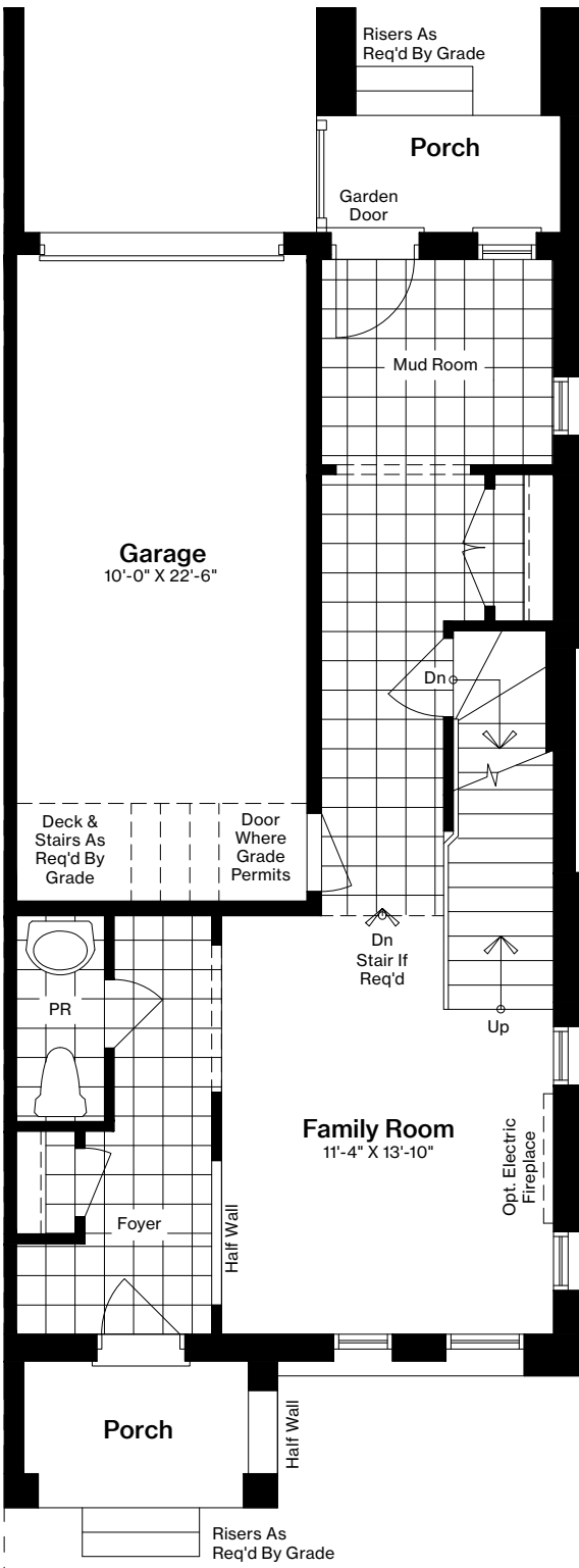
CORNER FIRST FLOOR PLAN
