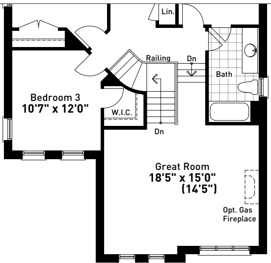
PARTIAL SECOND FLOOR PLAN ELEVATION C
