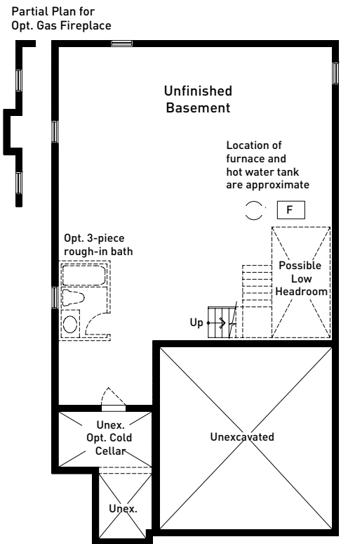
BASEMENT FLOOR PLAN ELEVATION A
