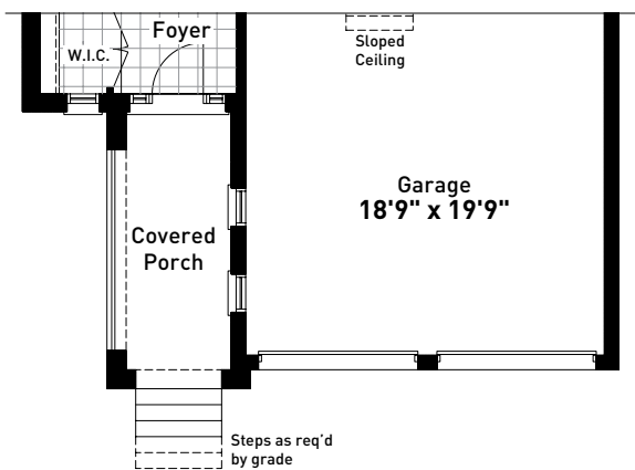
PARTIAL GROUND FLOOR PLAN ELEVATION C
