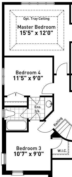
PARTIAL OPTIONAL SECOND FLOOR PLAN ELEVATION A
