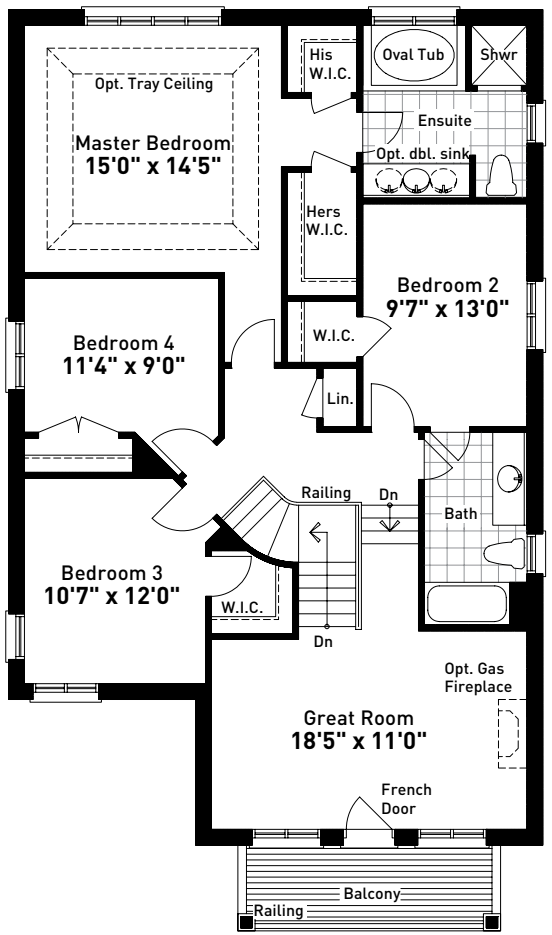
SECOND FLOOR PLAN ELEVATION B
