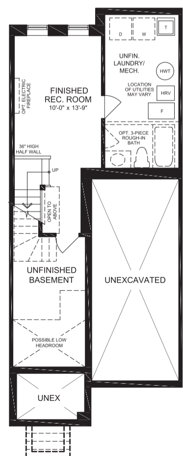
OPTIONAL FINISHED BASEMENT PLAN ELEVATION A
