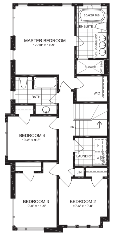
SECOND FLOOR PLAN ELEVATION B
