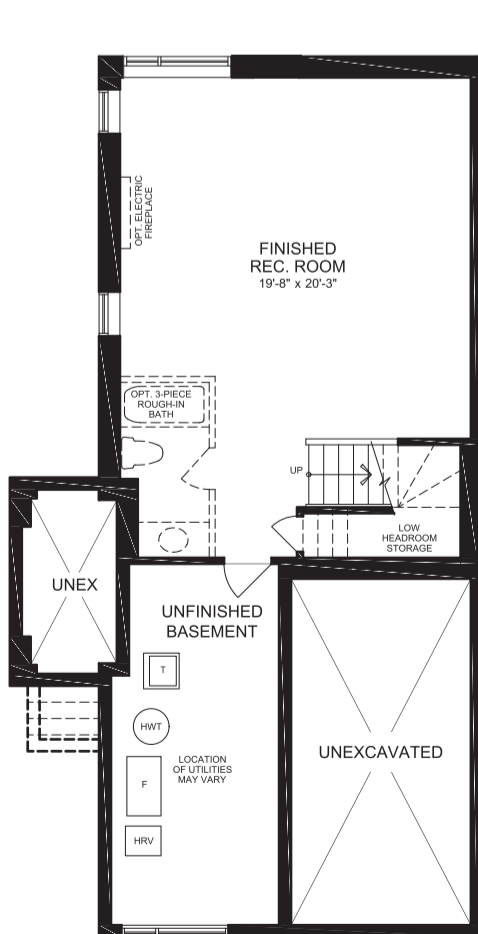
PARTIAL FINISHED BASEMENT PLAN W/ OPT. WALK-UP
