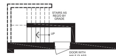
PARTIAL FINISHED BASEMENT PLAN W/ OPT. WALK-UP
