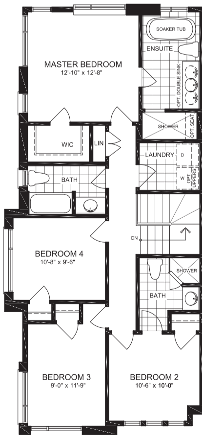
OPTIONAL SECOND FLOOR PLAN ELEVATION A
