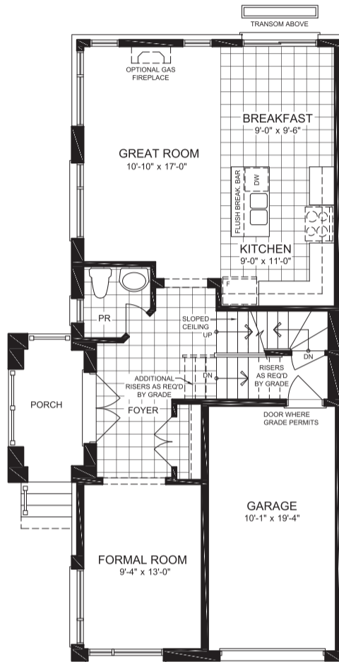
GROUND FLOOR PLAN ELEVATION A
