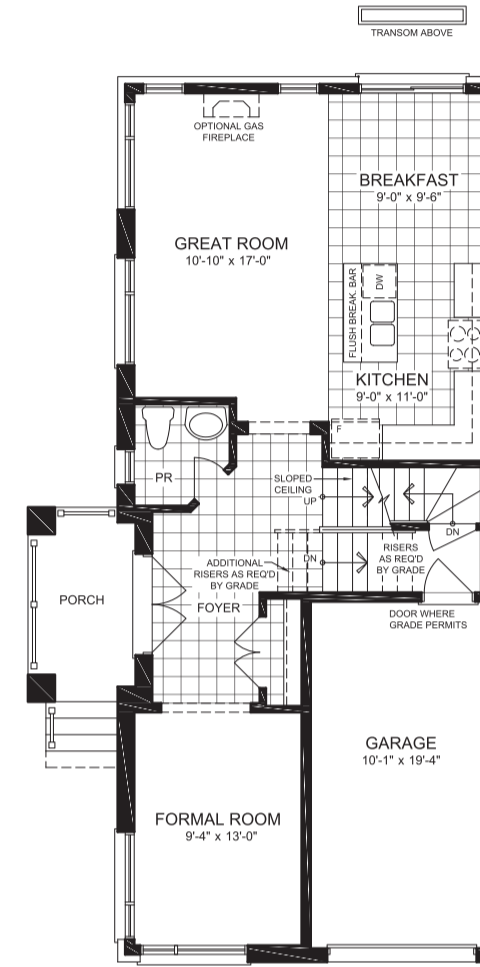
GROUND FLOOR PLAN ELEVATION B
