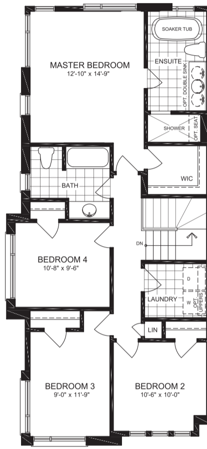
SECOND FLOOR PLAN ELEVATION A
