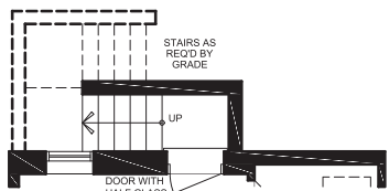
PARTIAL BASEMENT PLAN W/ OPT. WALK-UP
