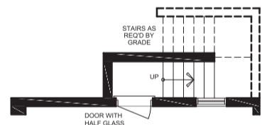
PARTIAL BASEMENT PLAN W/ OPT. WALK-UP
