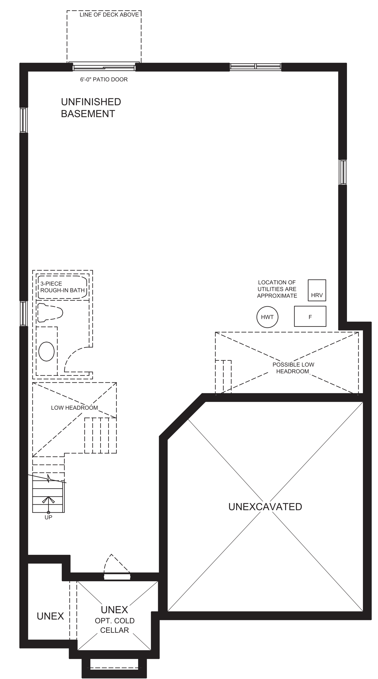
BASEMENT PLAN ELEVATION A
