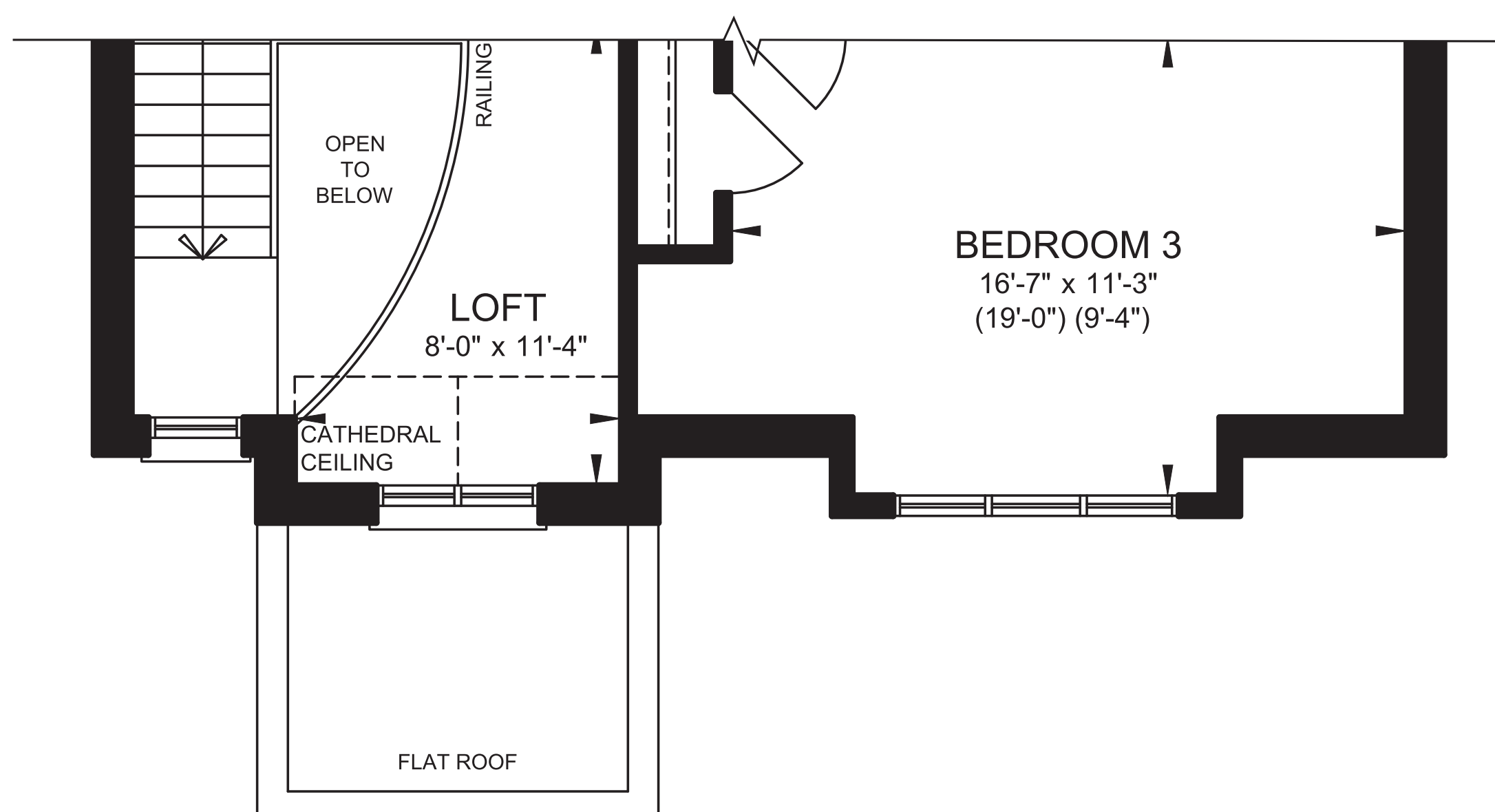
PARTIAL SECOND FLOOR PLAN ELEVATION B
