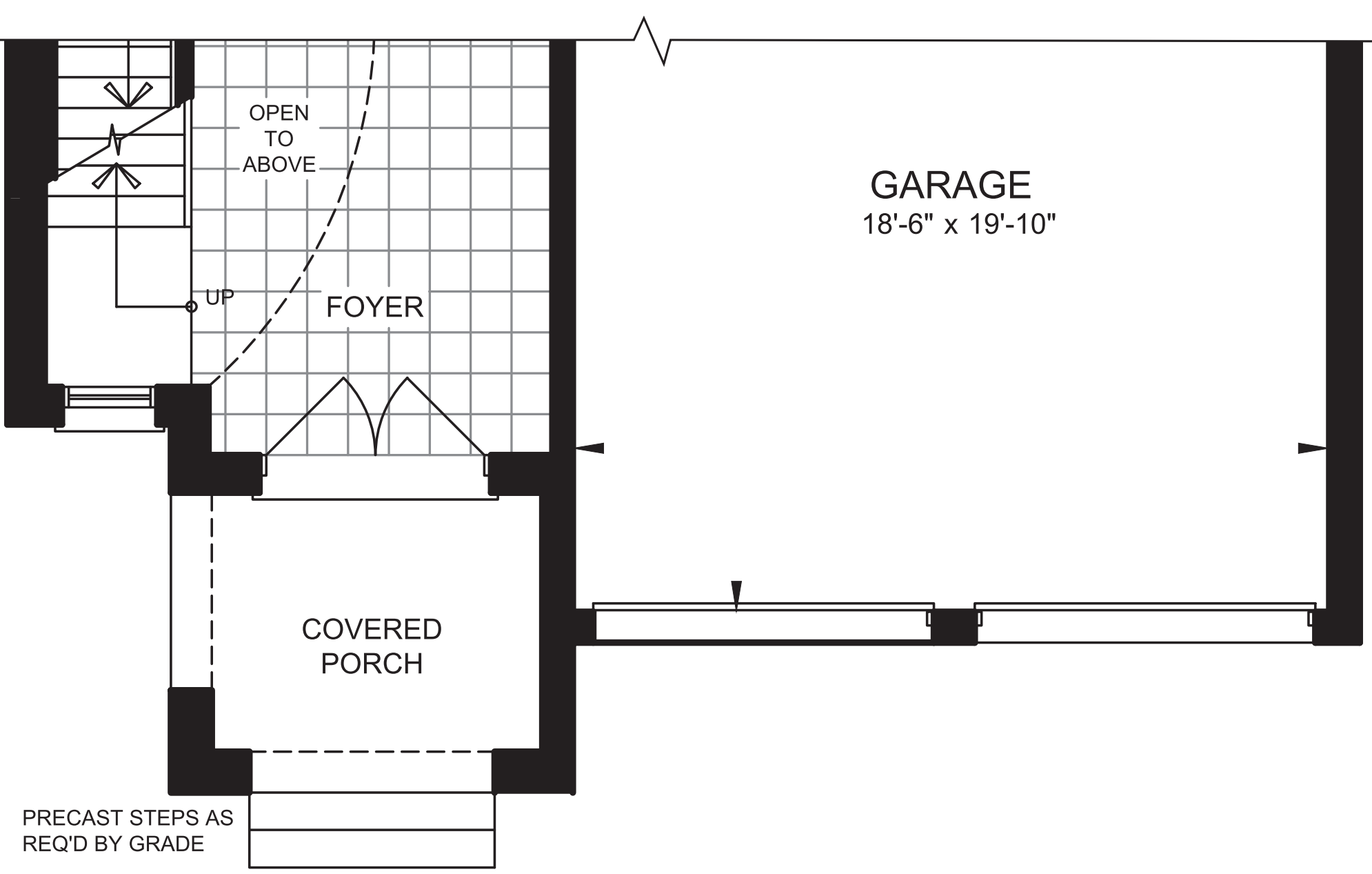
PARTIAL GROUND FLOOR PLAN ELEVATION B
