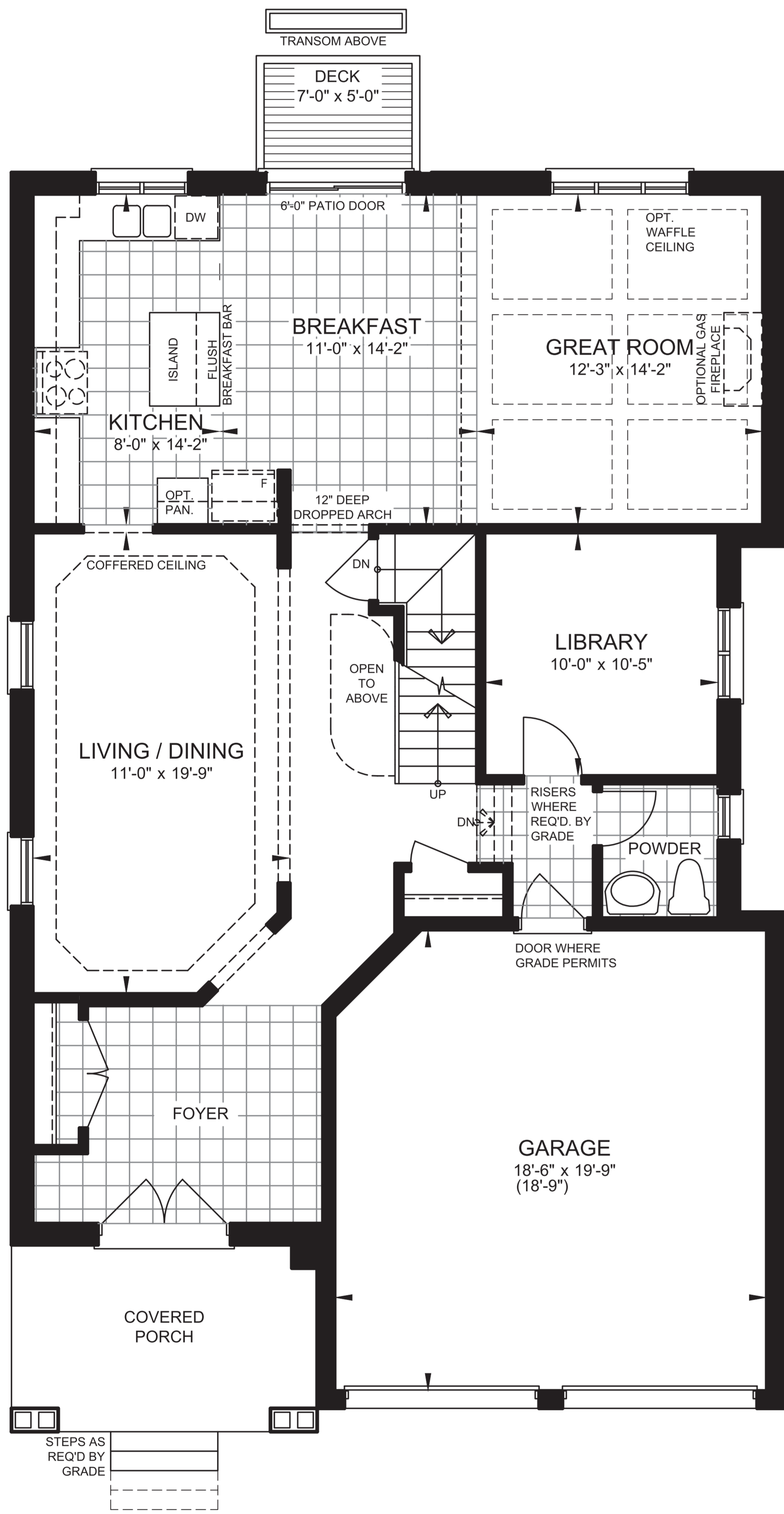
GROUND FLOOR PLAN ELEVATION A
