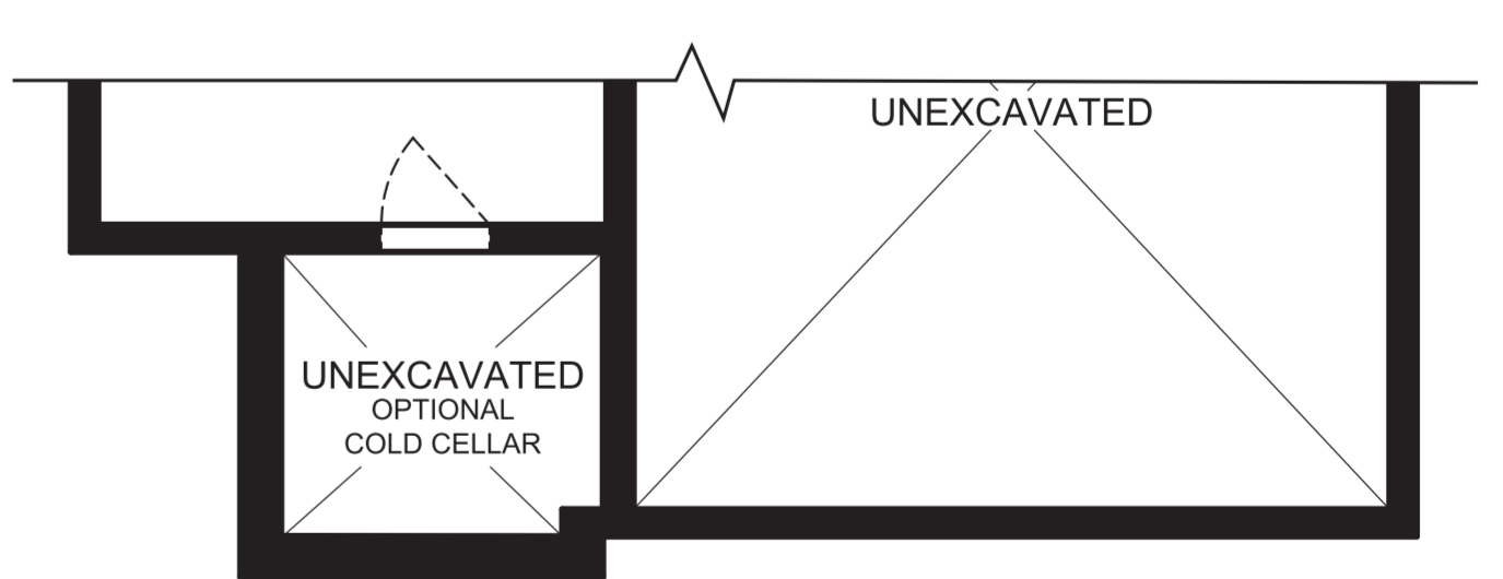
PARTIAL BASEMENT PLAN ELEVATION B
