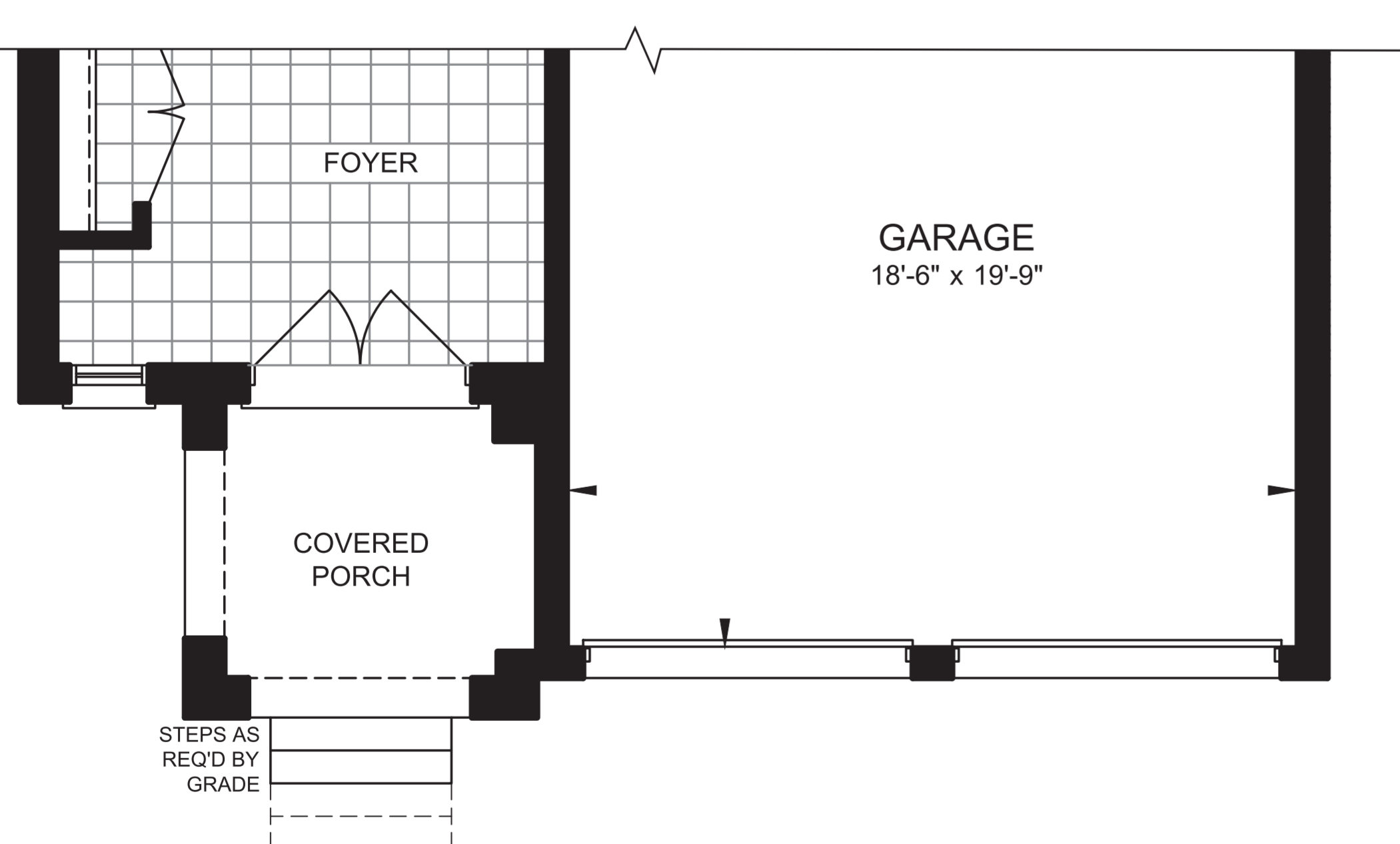
PARTIAL GROUND FLOOR PLAN ELEVATION B
