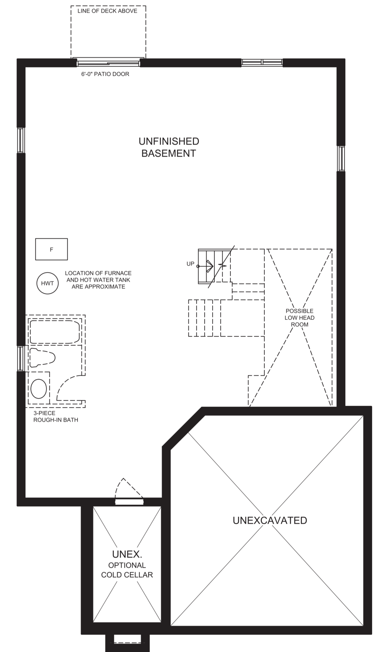
BASEMENT PLAN ELEVATION A
