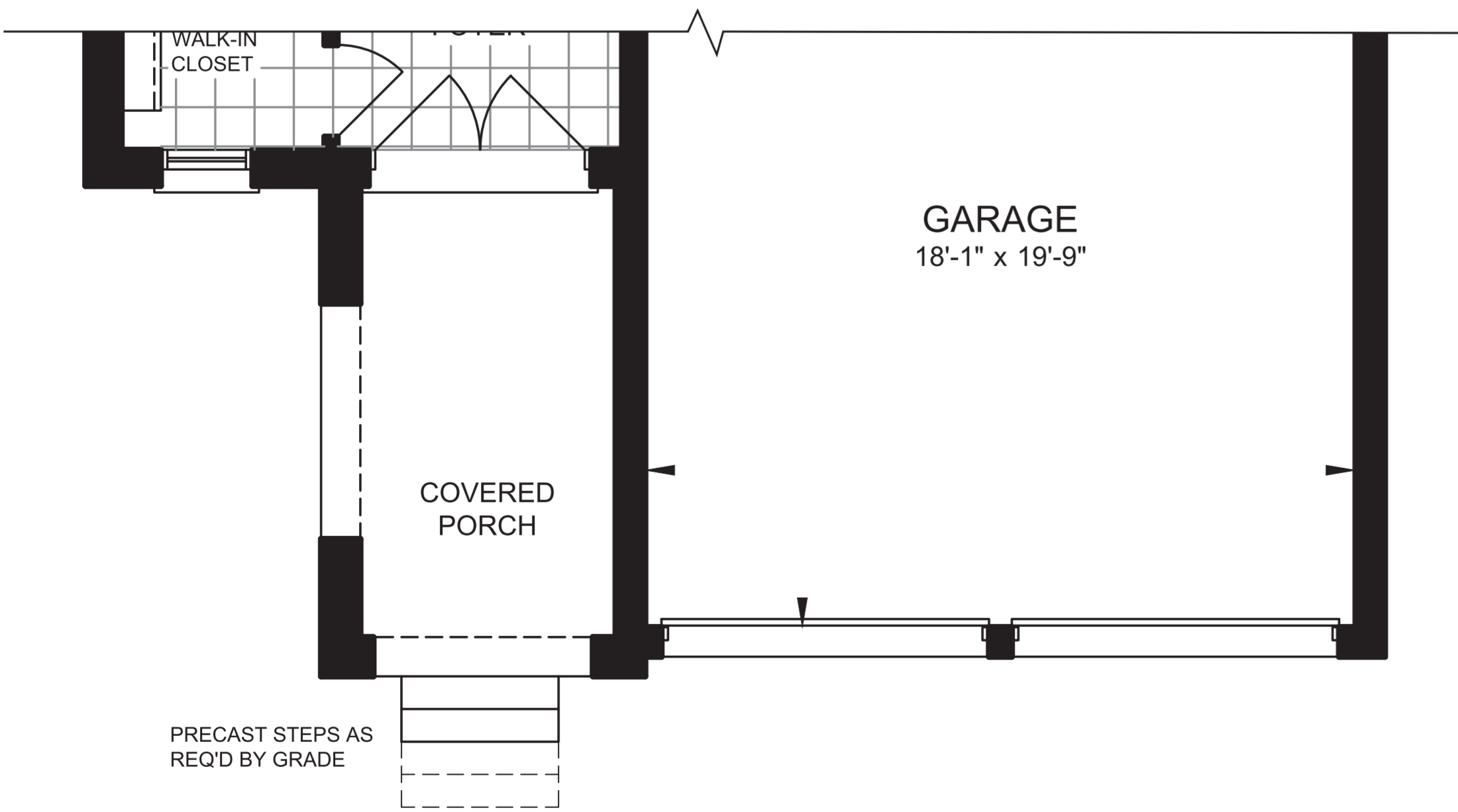
PARTIAL GROUND FLOOR PLAN ELEVATION B
