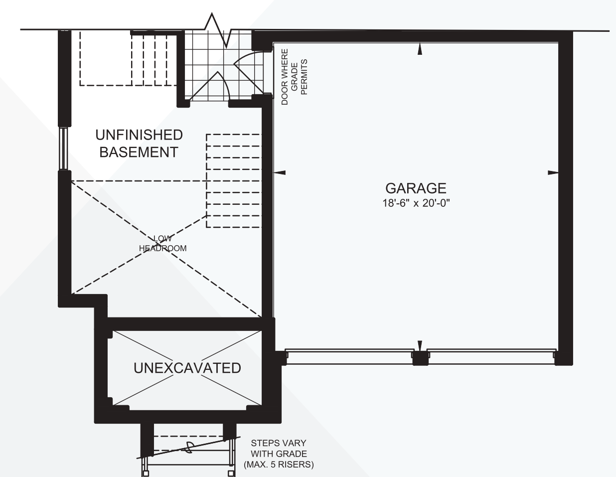
PARTIAL FINISHED BASEMENT PLAN ELEVATION B
