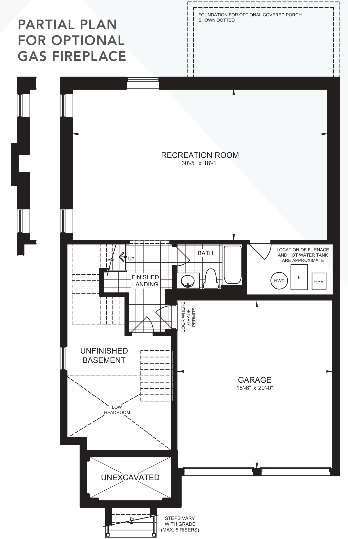
FINISHED BASEMENT PLAN ELEVATION A
