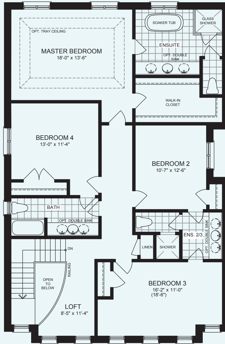
SECOND FLOOR PLAN ELEVATION A
