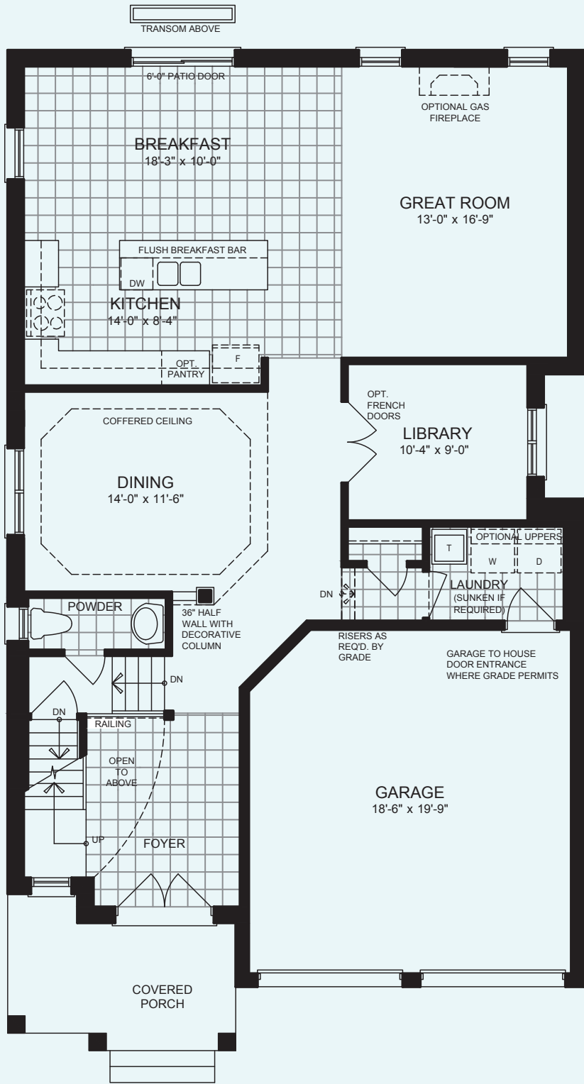
GROUND FLOOR PLAN ELEVATION A
