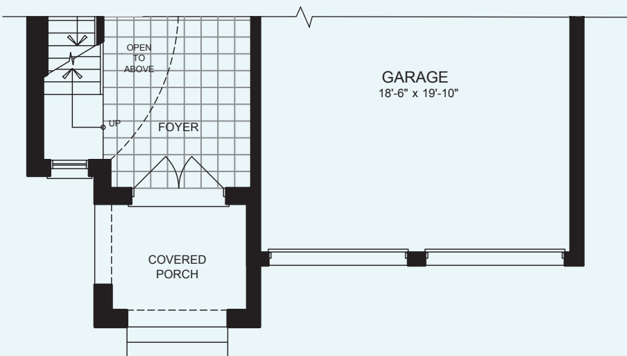
PARTIAL GROUND FLOOR PLAN ELEVATION B
