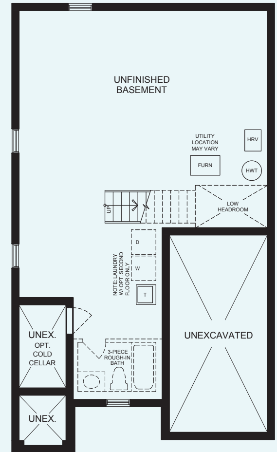
BASEMENT PLAN ELEVATION A
