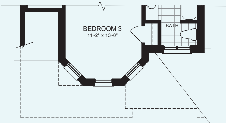
PARTIAL GROUND FLOOR PLAN ELEVATION B
