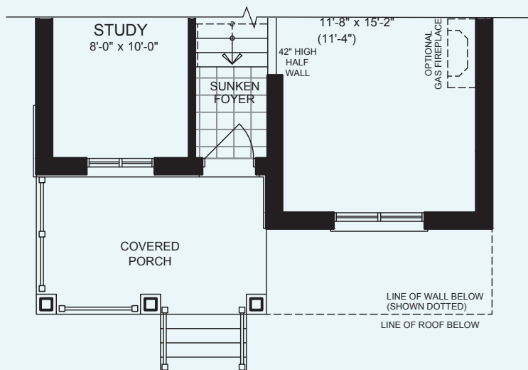
PARTIAL GROUND FLOOR PLAN ELEVATION B
