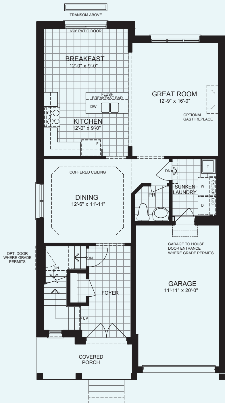
GROUND FLOOR PLAN ELEVATION A
