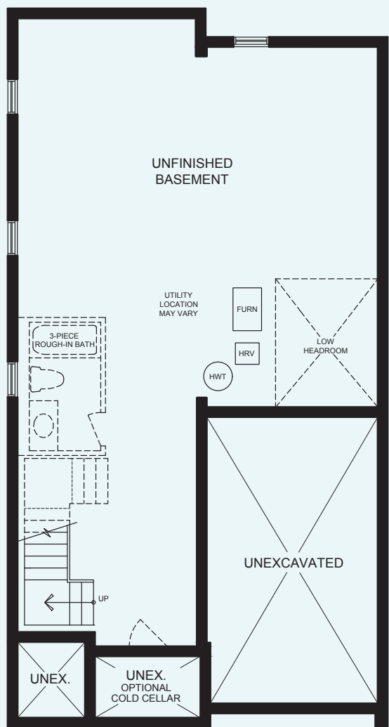
BASEMENT PLAN ELEVATION A
