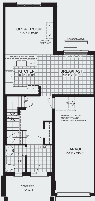
GROUND FLOOR PLAN ELEVATION A & B
