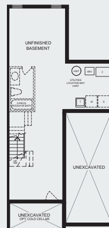
BASEMENT PLAN ELEVATION A & B
