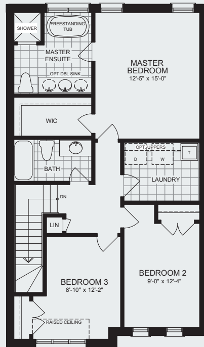
SECOND FLOOR PLAN ELEVATION A
