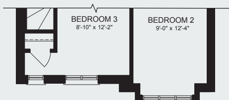
PARTIAL SECOND FLOOR PLAN ELEVATION B
