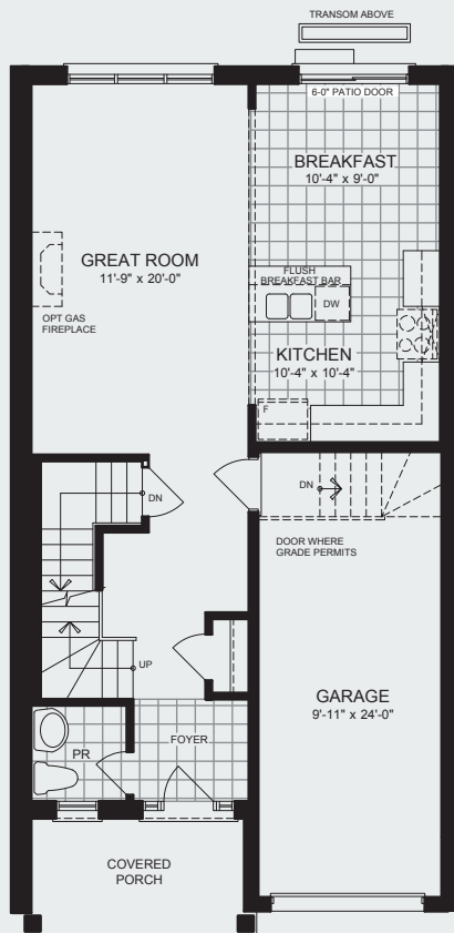
GROUND FLOOR PLAN ELEVATION A & B
