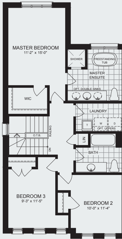
SECOND FLOOR PLAN ELEVATION A1
