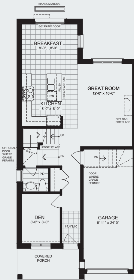
GROUND FLOOR PLAN ELEVATION A1, A2, & B
