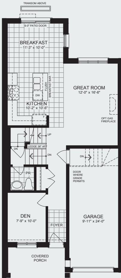
GROUND FLOOR PLAN ELEVATION A & B
