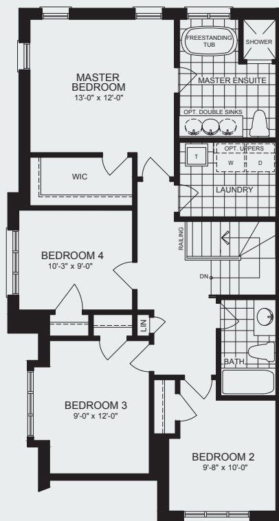
SECOND FLOOR PLAN ELEVATION B
