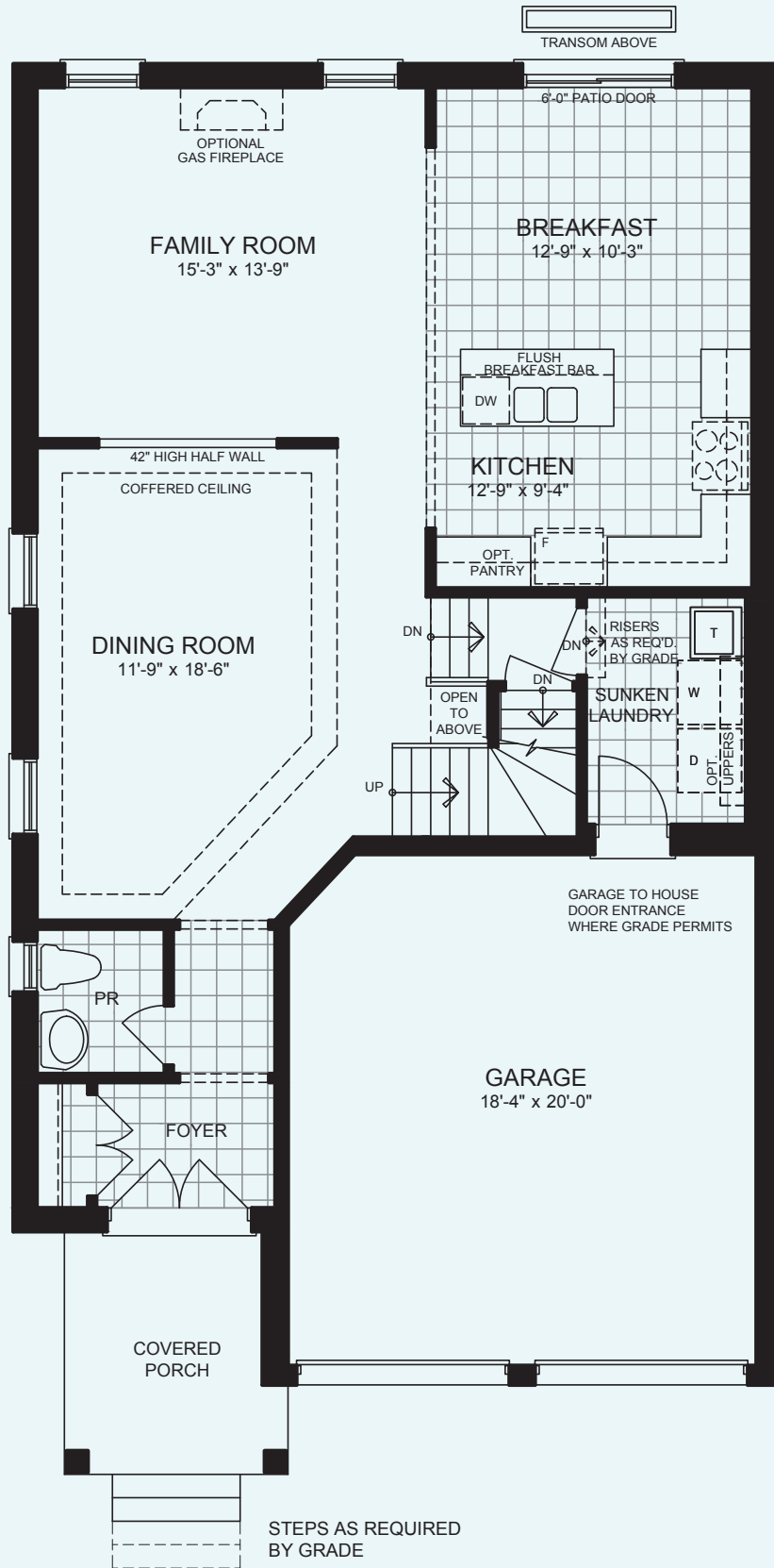
GROUND FLOOR PLAN ELEVATION A
